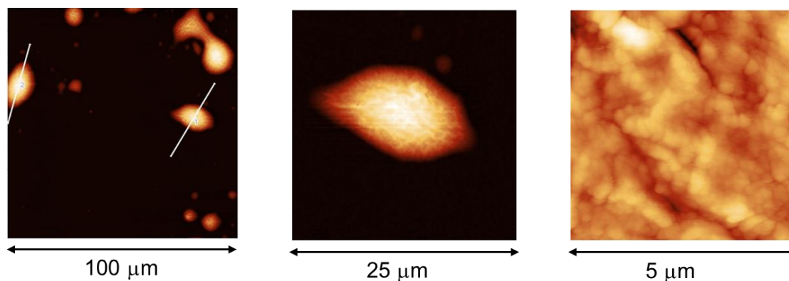
Figure 9. AFM images of different resolutions in size of the \text{CeO}_x layer annealed at 450^\circ\text{C} for 15 min showing crystalline clusters.
