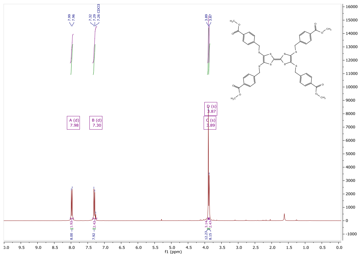
Figure S1. ^1\text{H} NMR (300 MHz, \text{CDCl}_3 ) spectra of 2
