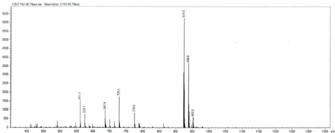
Figure S5. LRMS of 2.
