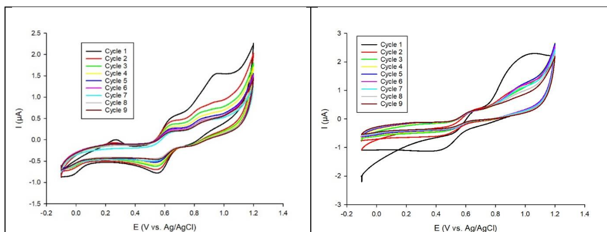
Figure S22. Solid-state cyclic voltammograms for \text{Cu}_8\text{L}_4\text{-(DMF)} (left) and \text{Cu}_8\text{L}_4\text{-(DMAc)} (right) recorded between -0.1 V and 1.2 V (WE: Pt; CE: Pt wire; RE: Ag/AgCl; electrolyte : 0.1 M TBAPF 6 in \text{CH}_3\text{CN} ; scan rate: 20 \text{mV}\cdot\text{s}^{-1} ).
