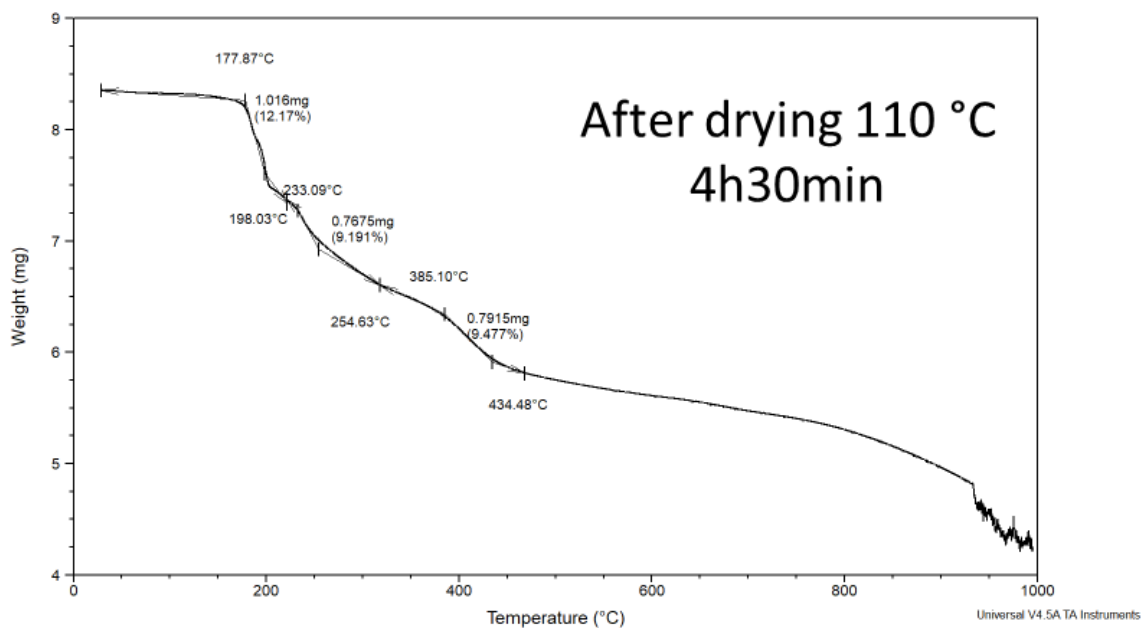
Figure S20. TGA after drying for \text{Cu}_8\text{L}_4\text{-(DMF)} .
