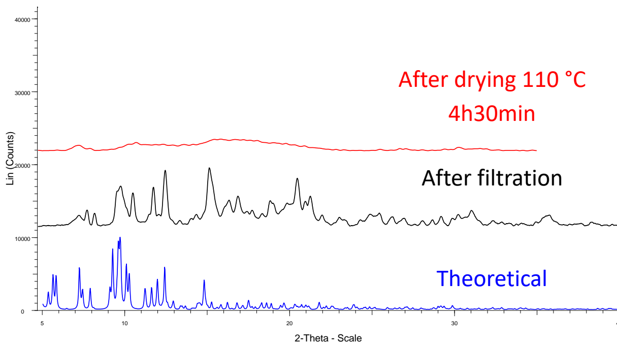
Figure S16. PXRD for \text{Cu}_8\text{L}_4\text{-(DMF)} .
