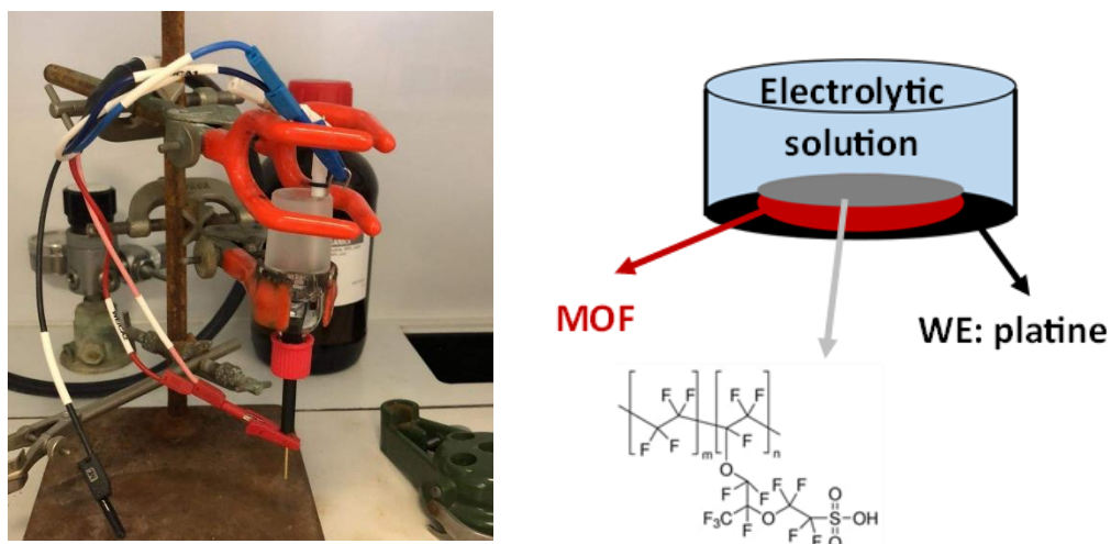
Figure S21. Solid state cyclic voltammetry set-up (left: set-up picture, right: schematic representation).
