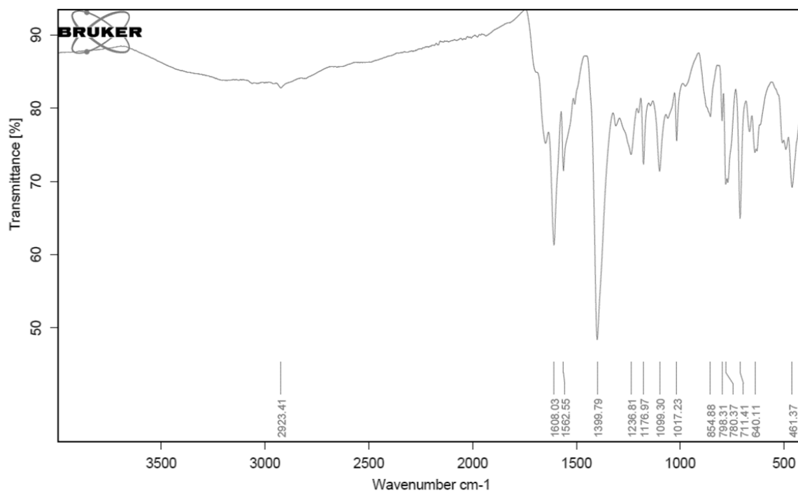
Figure S13. IR spectra of \text{Cu}_8\text{L}_4 -(DMF).
