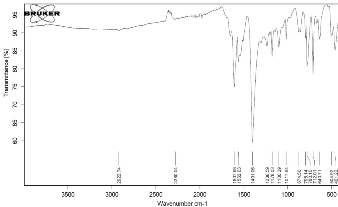
Figure S14. IR spectra of \text{Cu}_8\text{L}_4\text{-(DMF)} after drying.
