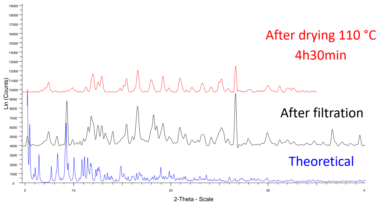
Figure S15. PXRD for \text{Cu}_8\text{L}_4\text{-(DMAc)} .
