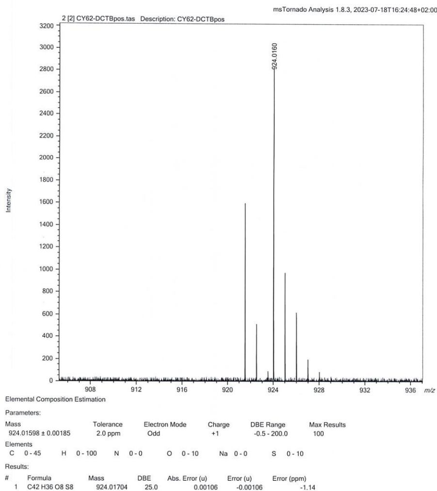
Figure S6. HRMS of 2.
