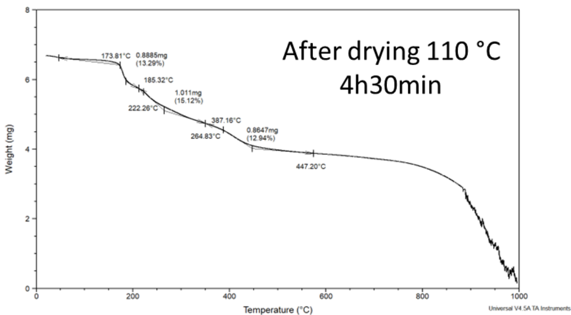
Figure S118. TGA after drying for \text{Cu}_8\text{L}_4\text{-(DMAc)} .
