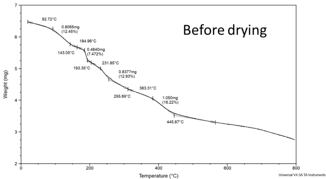
Figure S17. TGA before drying for \text{Cu}_8\text{L}_4\text{-(DMAc)} .
