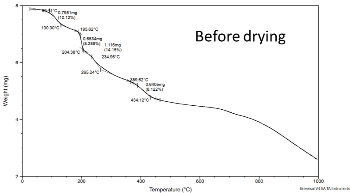
Figure S19. TGA before drying for \text{Cu}_8\text{L}_4\text{-(DMF)} .
