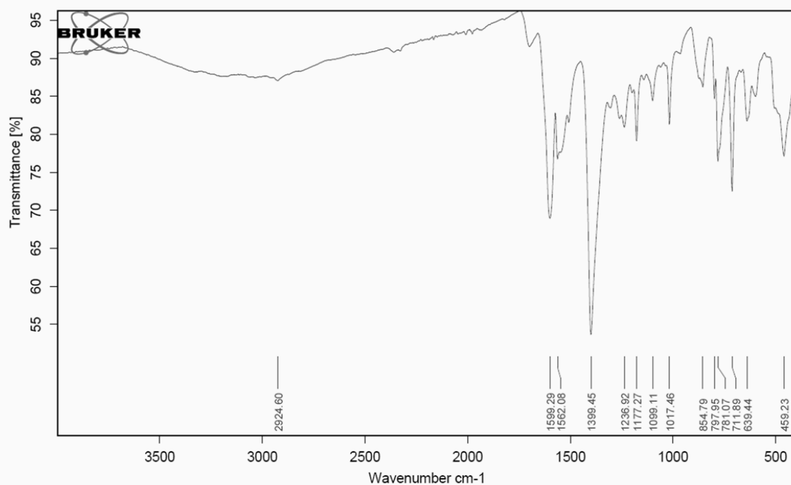
Figure S11. IR spectra of Cu 8 L 4 -(DMAc).
