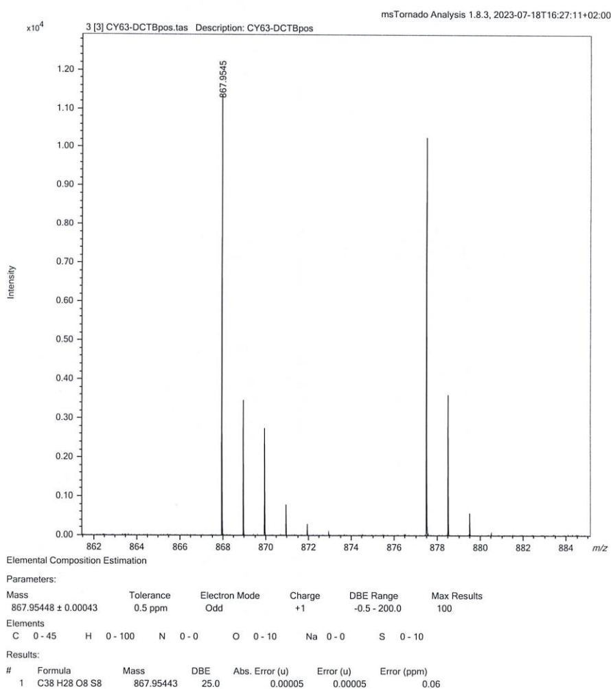
Figure S9. HRMS of L.
