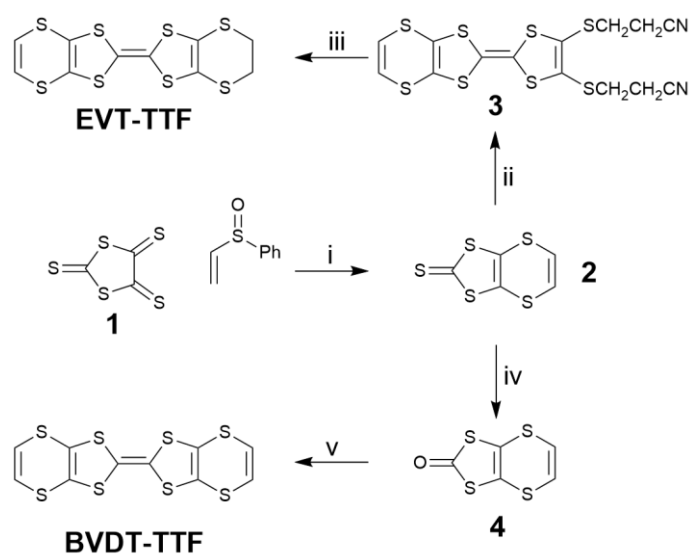
Scheme 1 Synthesis of BVDT-TTF and EVT-TTF . i) xylenes, \Delta ; ii) bis(thiopropionitrile)-dithiol-one, \text{P}(\text{OMe})_3 , \Delta ; iii) \text{EtONa} , \text{EtOH} , 1,2-dibromoethane; iv) \text{Hg}(\text{OAc})_2 , \text{CHCl}_3/\text{AcOH} , RT; v) \text{P}(\text{OMe})_3 , \Delta .
