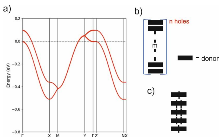
Fig. 7 (a) Band structure for the hypothetical metallic state of (BVDT-TTF) 2.5 (I 3 ) where \Gamma = (0, 0, 0) , X = (a^*/2, 0, 0) , Y = (0, b^*/2, 0) , Z = (0, 0, c^*/2) , M = (a^*/2, b^*/2, 0) and N = (a^*/2, 0, c^*/2) . Discrete (\text{donor}_m)^{n+} (b) and (\text{donor}_s)^{2+} (c) units discussed in the text.
