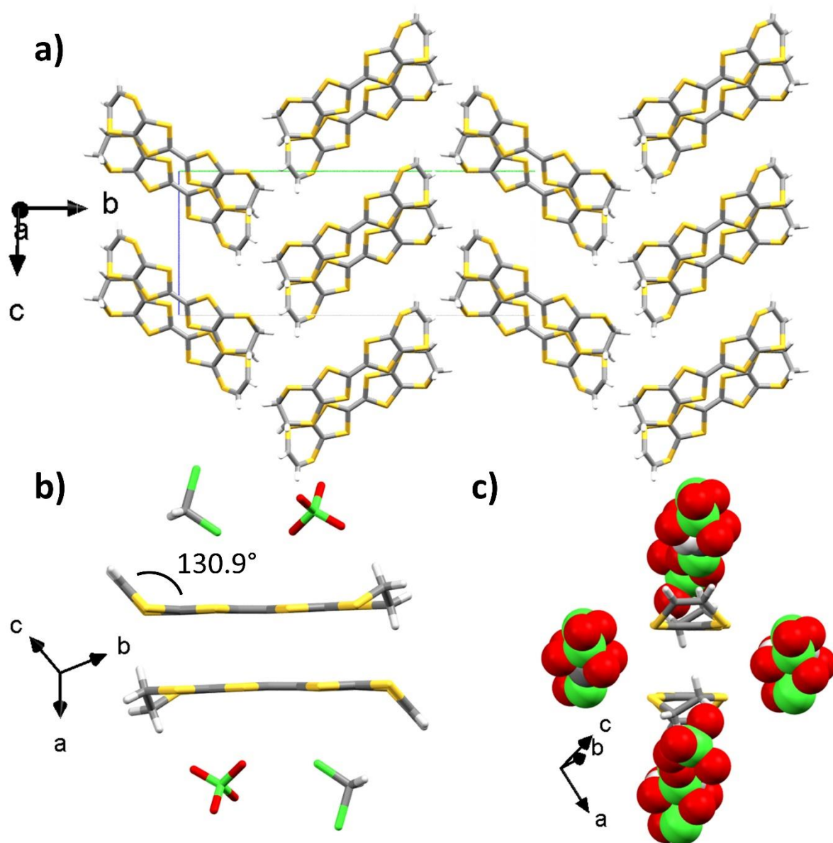
Fig. 4 X-ray crystal structure of (EVT-TTF)(ClO 4 )·0.5(CH 2 Cl 2 ) a) viewed along the a axis. Details showing b) a side-view of the EVT-TTF dimer and c) a front-view of the EVT-TTF dimer (For the sake of clarity, solvent molecules and anions have been omitted on (a), and disordered molecules have been omitted for the sake of clarity on (b) and (c) (Carbon: grey ; Sulphur : yellow ; Chlorine : green ; Oxygen : red ; Hydrogen : white) ).
