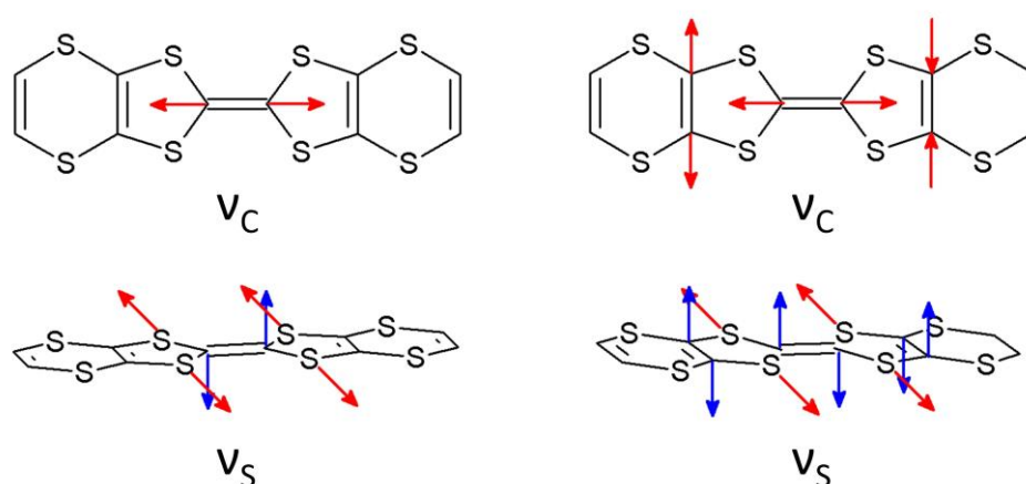
Fig. 10 The schematic patterns of the charge-sensitive C=C stretching \nu_C mode (upper panels) and the out-of-plane C-S stretching \nu_S mode (lower panels) of the BVDT-TTF •+ cation (left) and the EVT-TTF •+ cation (right), based on the DFT calculations.
