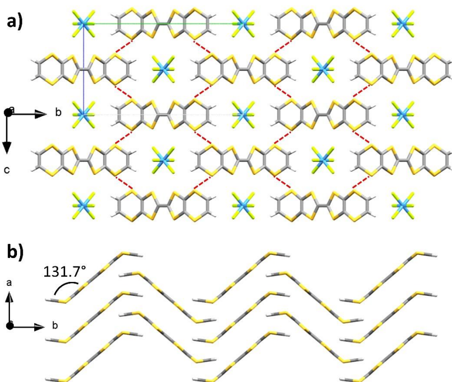
Fig. 1 X-ray crystal structure of BVDT-TTF(TaF 6 ) viewed along a) the a axis and b) the c axis (Carbon: grey ; Sulphur : yellow ; Tantalum : blue ; Fluorine : green ; Hydrogen : white). For the sake of clarity the TaF 6 - anions have been removed on b).
