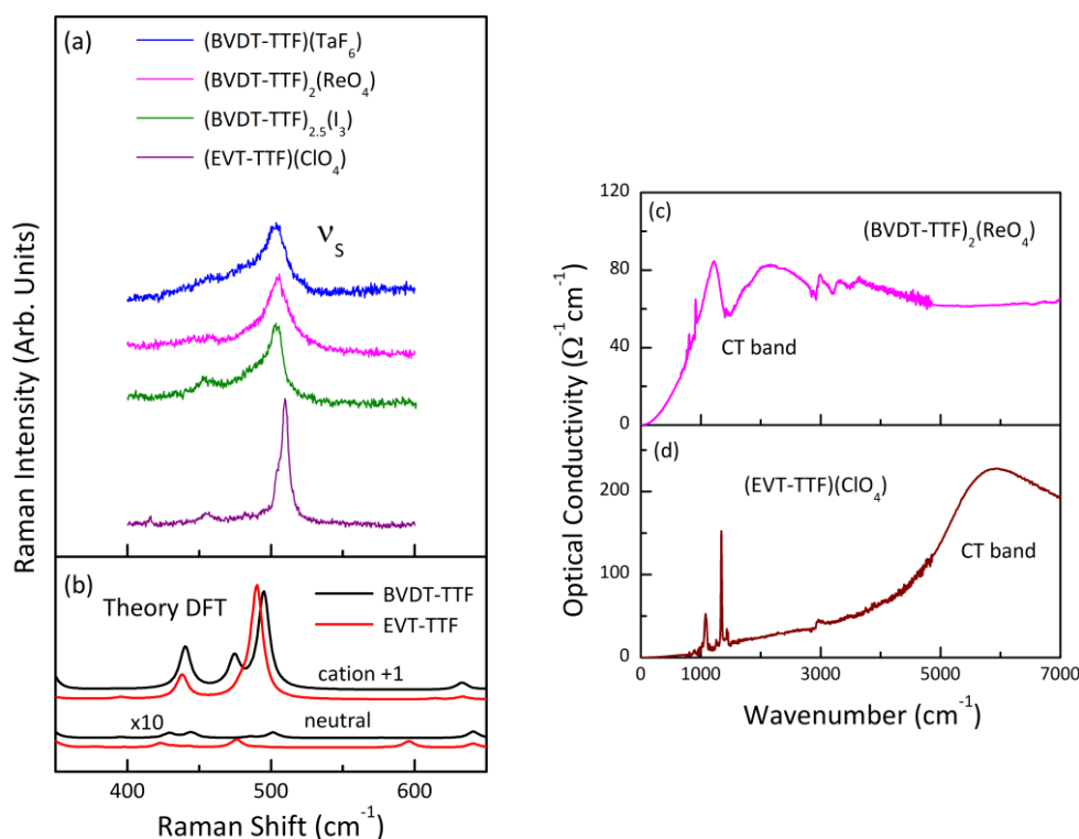
Fig. 12 (a) Raman spectra of (\text{BVDT-TTF})(\text{TaF}_6) , (\text{BVDT-TTF})_2(\text{ReO}_4) , (\text{BVDT-TTF})_{2.5}(\text{I}_3) , and (\text{EVT-TTF})(\text{ClO}_4) \cdot 0.5(\text{CH}_2\text{Cl}_2) measured at room temperature with the 632.8 nm excitation line, in the frequency range of the C=S stretching vibrations; (b) theoretical Raman spectra of the isolated BVDT-TTF and EVT-TTF donor molecules in their neutral and cationic forms, calculated at the B3LYP/6-31+ +G(d,p) level of theory; the theoretical spectra of the neutral BVDT-TTF and EVT-TTF have been multiplied by a factor of 10. The spectra in panels (a,b) are offset for clarity; (c) room temperature optical conductivity spectra of (\text{BVDT-TTF})_2(\text{ReO}_4) , and (\text{EVT-TTF})(\text{ClO}_4) \cdot 0.5(\text{CH}_2\text{Cl}_2) , respectively, polarized in the conducting plane.
