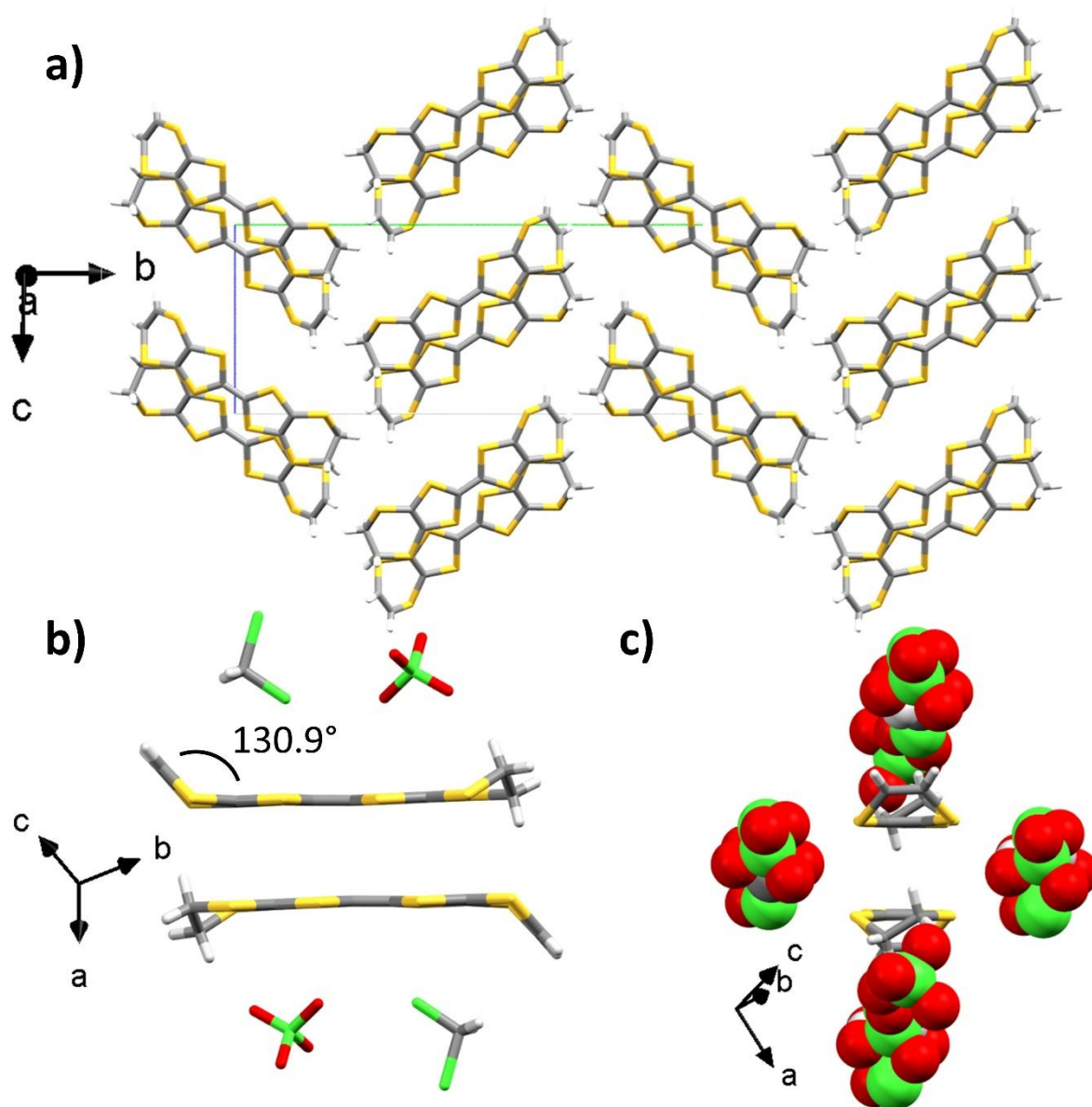
Fig. 4 X-ray crystal structure of (\text{EVT-TTF})(\text{ClO}_4) \cdot 0.5(\text{CH}_2\text{Cl}_2) a) viewed along the a axis. Details showing b) a side-view of the EVT-TTF dimer and c) a front-view of the EVT-TTF dimer (For the sake of clarity, solvent molecules and anions have been omitted on (a), and disordered molecules have been omitted for the sake of clarity on (b) and (c) (Carbon: grey ; Sulphur : yellow ; Chlorine : green ; Oxygen : red ; Hydrogen : white) ).
