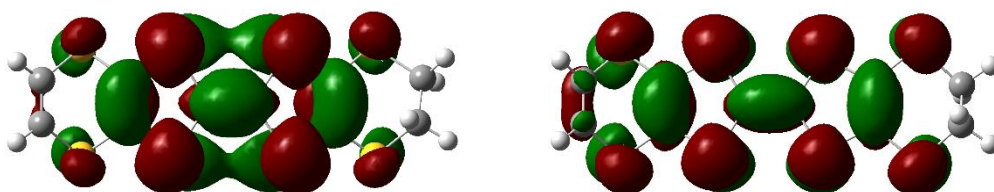
Fig. 9 Frontier molecular orbitals: HOMO (Highest Occupied Molecular Orbital) of the neutral EVT-TTF (left), and \alpha -SOMO (Single Occupied MO) of the EVT-TTF •+ radical cation (right), calculated by DFT methods.
