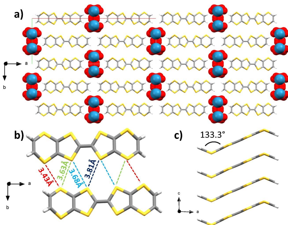
Fig. 3 X-ray crystal structure of (BVD-TTF) 2 (ReO 4 ) a) viewed along the c axis. Details showing b) the intermolecular S-S distances between two molecules from adjacent stacks viewed along the c axis, and c) a side-view along the b axis of one stack of BVD-TTF (Carbon: grey ; Sulphur : yellow ; Rhenium : blue ; Oxygen : red ; Hydrogen : white).
