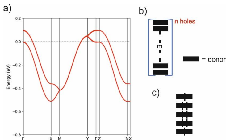
Fig. 7 (a) Band structure for the hypothetical metallic state of (BVDT-TTF) 2.5 (I 3 ) where \Gamma = (0, 0, 0) , X = (a^*/2, 0, 0) , Y = (0, b^*/2, 0) , Z = (0, 0, c^*/2) , M = (a^*/2, b^*/2, 0) and N = (a^*/2, 0, c^*/2) . Discrete ( \text{donor}_m ) n+ (b) and ( \text{donor}_s ) 2+ (c) units discussed in the text.
