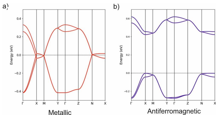
Fig. 6 Band structure for the (a) metallic and (b) antiferromagnetic (along a ), states of BVDT-TTF(TaF 6 ) using a double cell along a . The energy zero refers to the highest occupied state in both cases and \Gamma = (0, 0, 0) , X = (a^*/2, 0, 0) , Y = (0, b^*/2, 0) , Z = (0, 0, c^*/2) , M = (a^*/2, b^*/2, 0) and N = (a^*/2, 0, c^*/2) . In (b) the spin-up and spin-down bands are shown in blue and red, respectively. However, since the spin-up and spin-down bands are identical, although located in spatially different but equivalent sites, they superpose and only the blue bands are visible.
