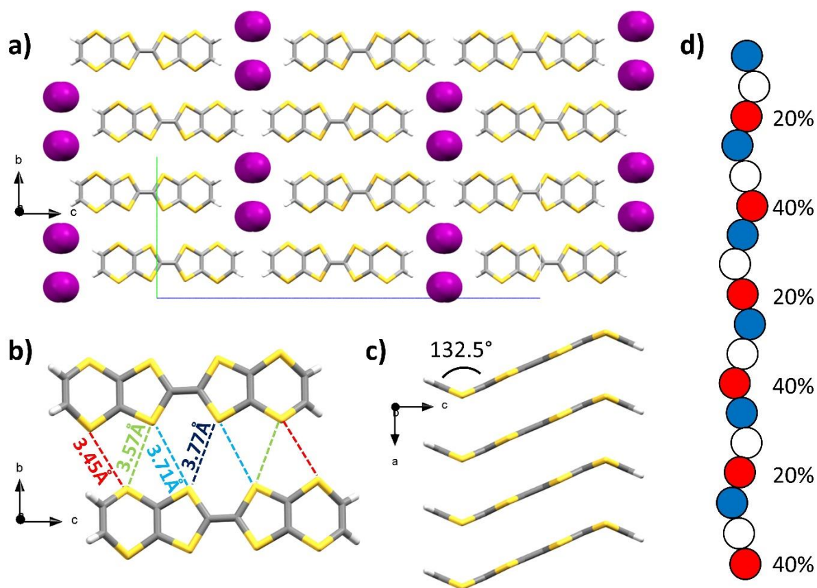
Fig. 2 X-ray crystal structure of (\text{BVD-TTF})_{2.5}(\text{I}_3) a) viewed along the a axis. Details showing b) the intermolecular S-S distances between two molecules from adjacent stacks viewed along the a axis, c) a side-view along the b axis of a single stack of BVD-TTF and d) a schematized view of the disorder of the triiodide counter-anions along the b axis (Carbon: grey; Sulphur: yellow; Iodine: purple; Hydrogen: white).
