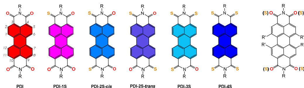
Figure 1. Representation of perylene-3,4,9,10-tetracarboxylic diimide (PDI) and its thionated derivatives.
