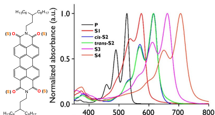
Figure 4. Normalized optical absorption spectra in \text{CHCl}_3 solution of PDI ( P ) and its corresponding thionated derivatives PDI-1S ( S1 ), PDI-2S-cis ( cis-S2 ), PDI-2S-trans ( trans-S2 ), PDI-3S ( S3 ) and PDI-4S ( S4 ). Reproduced with permission from reference [40]. Copyright 2014 American Chemical Society.
