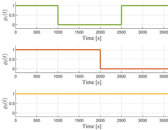
Fig. 3. Illustrations of \phi_1(t) , \phi_2(t) and \phi_3(t) .
