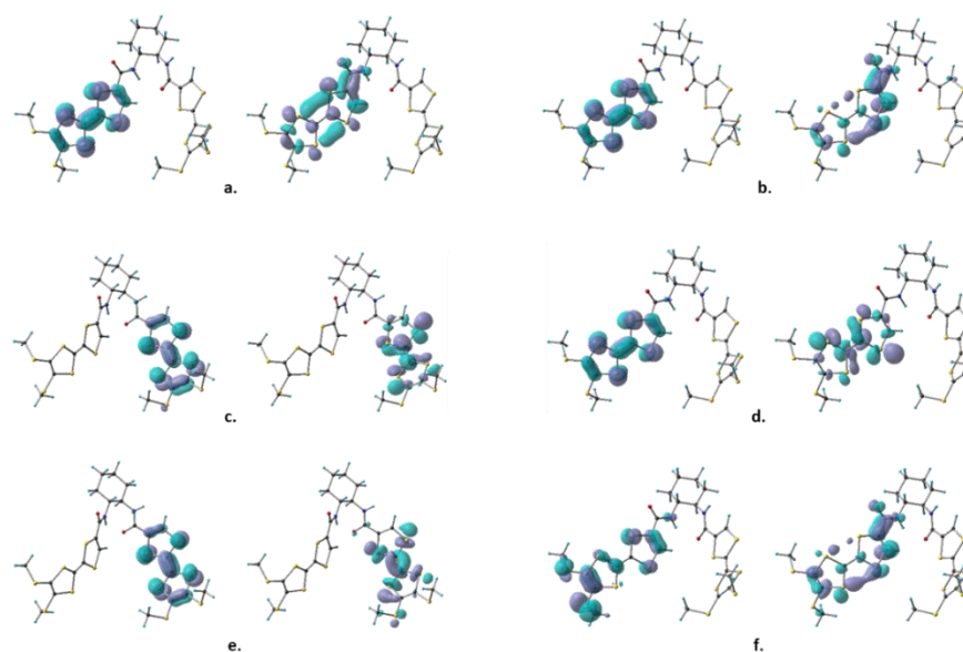
Figure 13. NTOs computed for the neutral ( R,R )-1 enantiomer, describing the following mono-electronic excitations: (a) S_0 \rightarrow S_2 , (b) S_0 \rightarrow S_4 , (c) S_0 \rightarrow S_{13} , (d) S_0 \rightarrow S_{14} , (e) S_0 \rightarrow S_{16} and (f) S_0 \rightarrow S_{25} .
