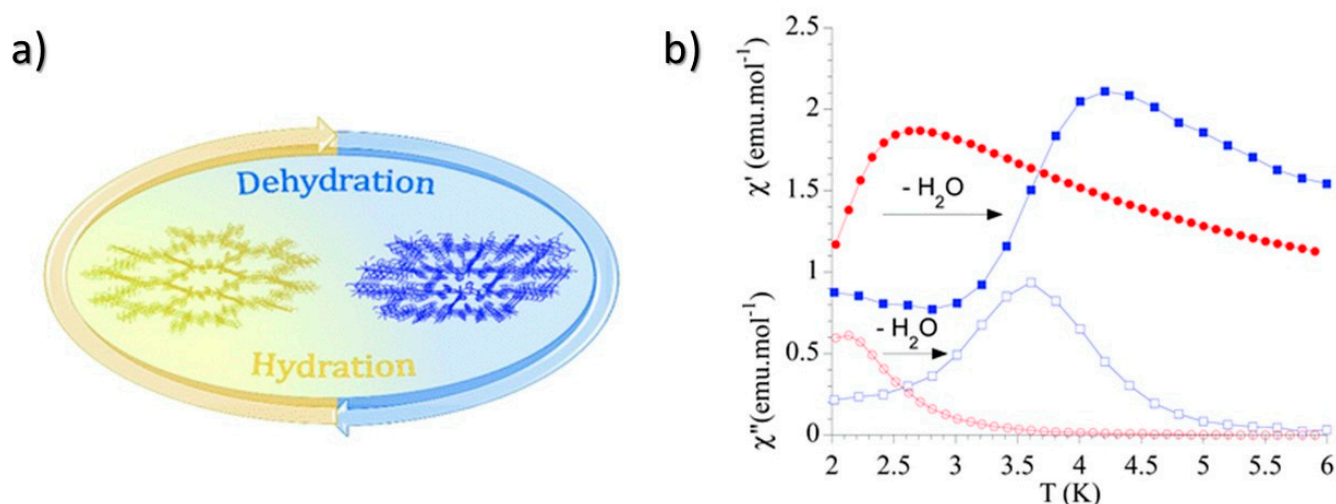
Figure 6. (a) Reversible expansion/shrinkage from hexagonal distorted cavities in 14a to distorted 3,6-brickwall rectangular cavities in 14a_des (left); (b) plot of \chi' and \chi'' vs T of 14a (full and empty red circles, respectively and 14a_des full and empty blue circles) under an applied dc field of 0.09 T at 10,000 Hz. Adapted with permission from [40].
