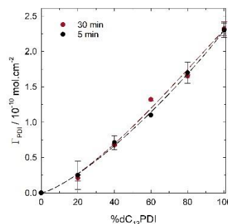
Figure 3. Surface coverages of PDI determined from the integration of CVs shown in Figure 2 vs the percentage of d\text{C}_{12}\text{PDI} in the grafting solution. The black markers represent the surface coverages obtained by reduction at 0 V for 5 min, while the red markers represent the surface coverages obtained by reduction at 0 V for 30 min.
