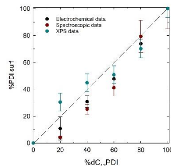
Figure 7. Percentage of PDI on the surface, indicated by green markers (calculated from XPS data), black markers (calculated from electrochemical data) and red markers (calculated from spectroscopic data), plotted as a function of the percentage of dC_{12}PDI in the grafting solution.
