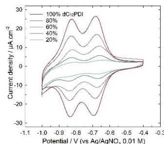
Figure 2. CVs recorded at 100 mV.s -1 for mixed C 12 PDI/C 12 Br-based layers obtained by reduction at 0 V for 5 min in a solution containing dC 12 PDI/dC 12 Br molar ratios of 100/0, 80/20, 60/40, 40/60, 20/80. The electrolyte used was 0.1 M nBu 4 NPF 6 in DCM and the total concentration of (dC 12 PDI + dC 12 Br) was 10 -3 M.
