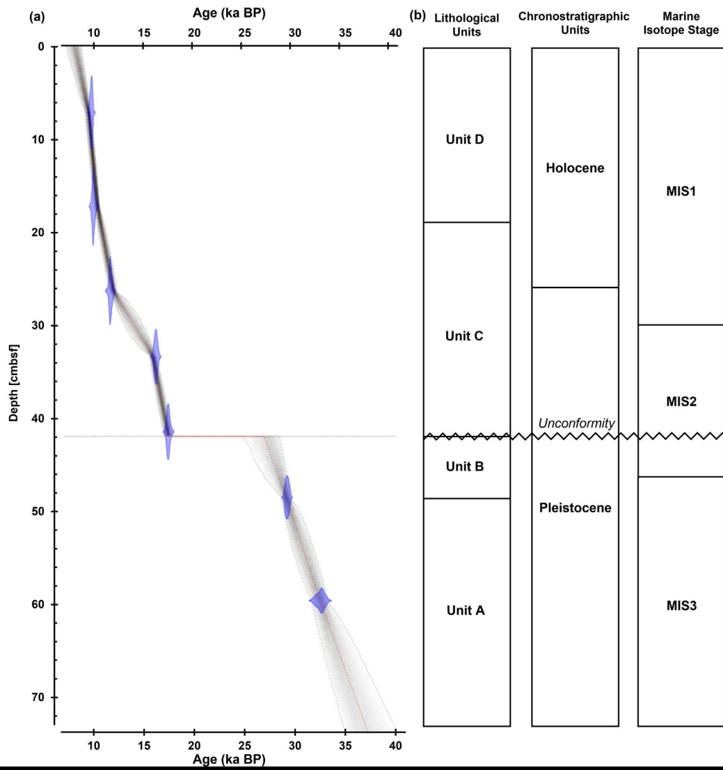
Fig. 4. (a) Age model established with RBacon using 7 AMS 14 C dates. (b) Subsequent classification of core CE18011_VC2 versus depth.
