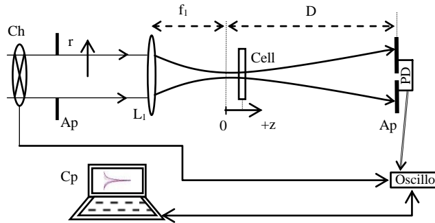
Fig. 1: Scheme showing the different position of the optical elements. The cell is scanned along the beam direction around the focal plane ( z=0 ). The labels refer to: lens ( L_1 ), chopper (Ch), circular aperture (Ap), computer (Cp) and photodiode (PD).
