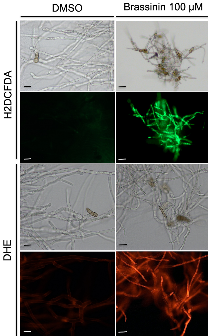
FIGURE 6 | Assessment of oxidative stress within A. brassicicola cells exposed for 30 min to 100 \mu\text{M} brassinin or to DMSO. The fluorescent dyes \text{H}_2\text{DCFDA} and DHE were used to detect the accumulation of ROS within hyphae of germlings treated for 1 h with DMSO (control) or 100 \mu\text{M} brassinin. For each panel, the bottom part corresponds to fluorescence microscopy and the top part to light-field microscopy. Scale bars = 20 \mu\text{m} .
