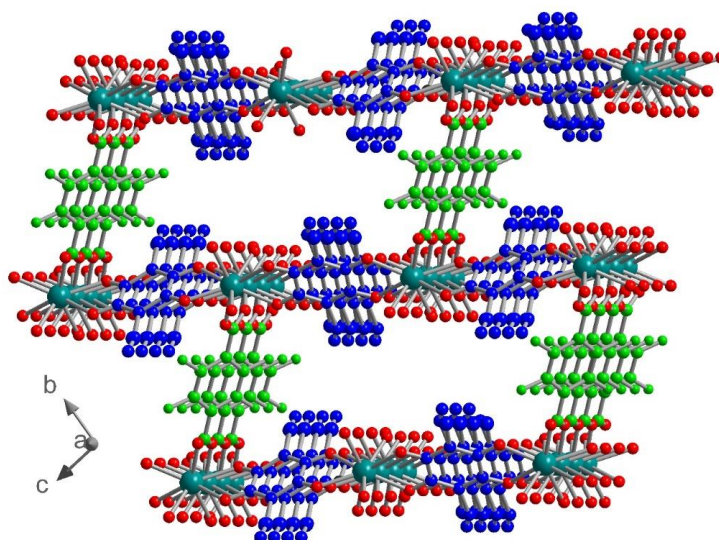
Figure 3. View of the crystal structure in 1 showing the rectangular cavities along the a axis. CICNAn 2- and F 4 BDC 2- are highlighted in blue and green respectively.
