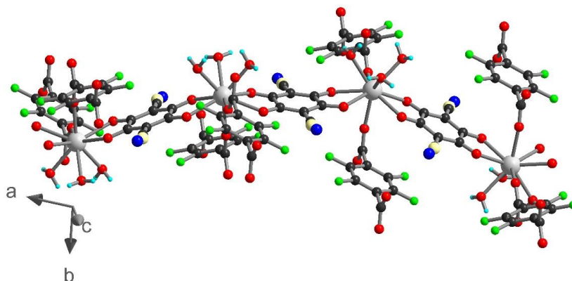
Figure 5. 1D chain of \text{Eu-ClCNAn}^{2-} connected by \text{F}_4\text{BDC}^{2-} ligands in 3 . Color code: C (black), H (cyan), O (red), N (blue), F (green), Cl (light yellow), Eu (grey).
