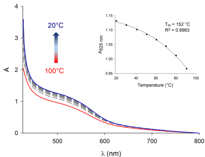
Figure 5. Evolution of the visible absorption spectrum of a C_3Pyr/C_3NDI (1:1) mixture in TCE ( [C_3Pyr] = [C_3NDI] = 5.2 mM) upon decreasing the temperature from 100 °C (red curve) to 20 °C (blue curve) (interval of 10 °C between each curve). Inset. Corresponding evolution of the absorbance at \lambda = 525 nm.
