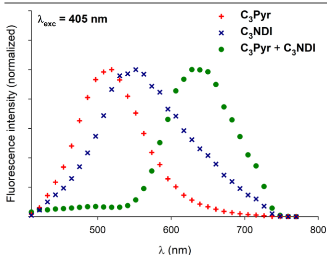
Figure 9. Normalized emission spectra of xerogels prepared by gel deposition of individual compounds C 3 Pyr (8 mg/mL), C 3 NDI (10 mg/mL) and their equimolar mixture C 3 Pyr/C 3 NDI (identical concentrations) in TCE for \lambda_{\text{exc}} = 405 nm.
