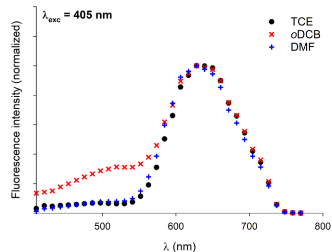
Figure 10. Normalized emission spectra of xerogels prepared by gel deposition of C 3 Pyr/C 3 NDI (1:1) mixtures in TCE, oDCB, and DMF for \lambda_{\text{exc}} = 405 nm.
