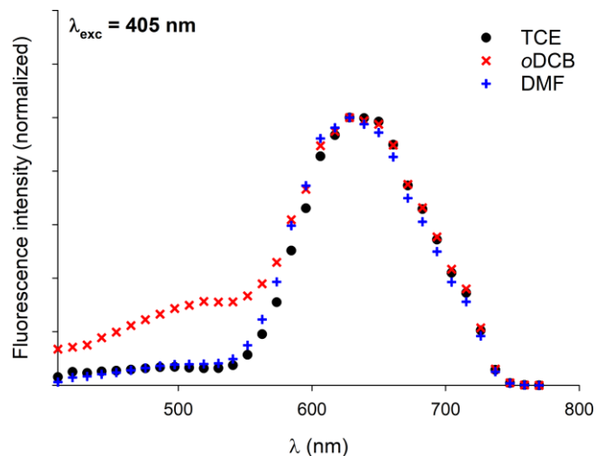
Figure 10. Normalized emission spectra of xerogels prepared by gel deposition of C_3Pyr/C_3NDI (1:1) mixtures in TCE, o DCB, and DMF for \lambda_{exc} = 405 nm.
