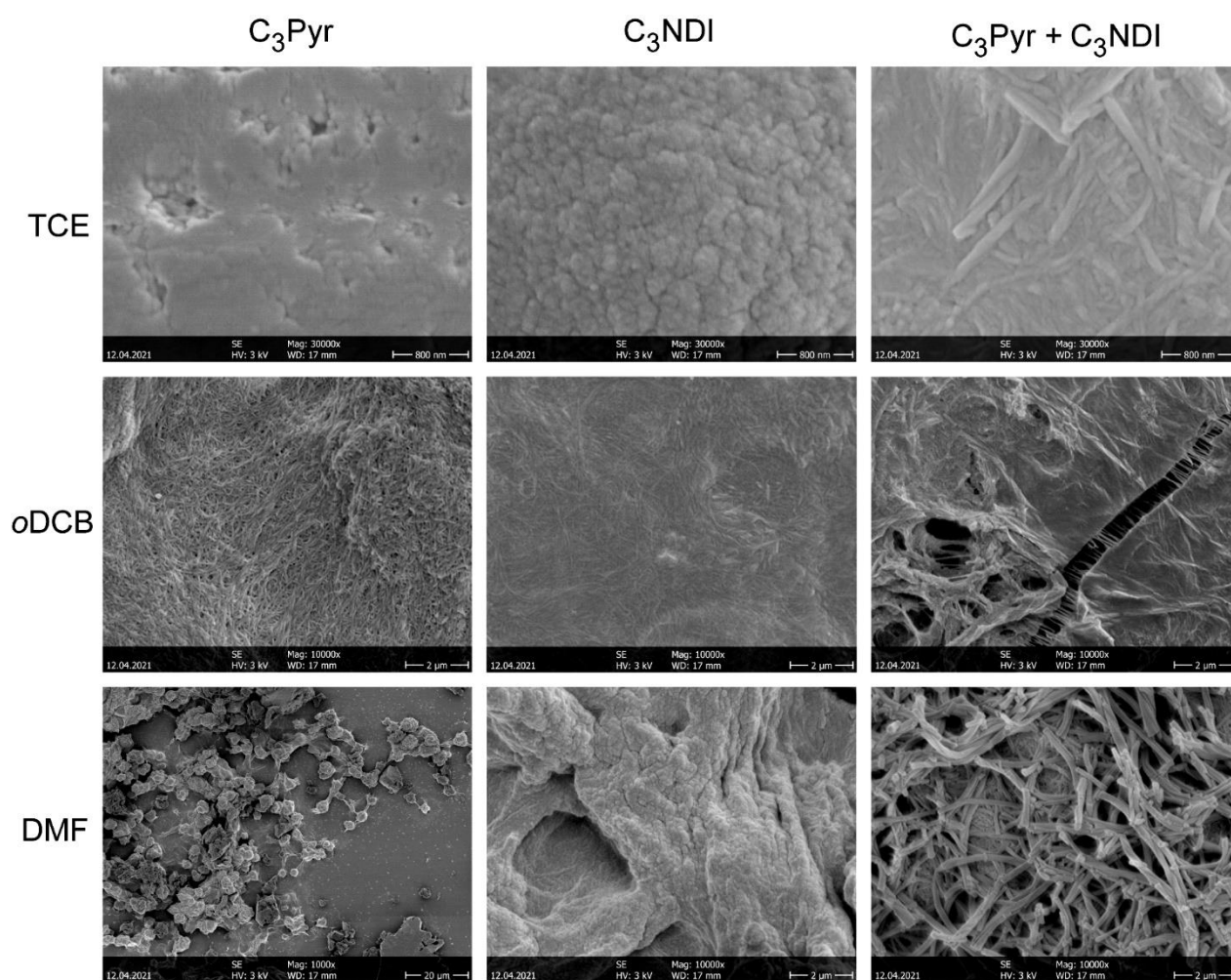
Figure 6. SEM micrographs of samples prepared by gel deposition of the individual compounds C 3 Pyr (8 mg/mL, a), C 3 NDI (10 mg/mL, b) and their equimolar mixture C 3 Pyr/C 3 NDI (identical concentrations, c) in TCE.
