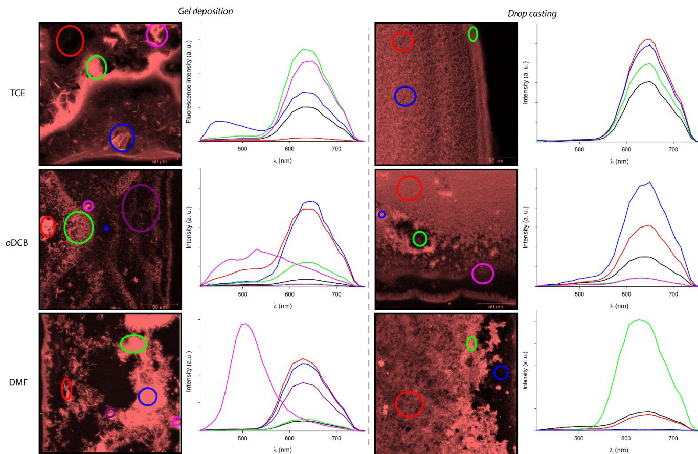
Figure 11. Emission spectra of the whole images (black line) and specific areas (highlighted with different colours in the corresponding images) obtained by confocal microscopy of xerogels prepared by gel deposition (a) or by drop casting hot solution (b) of the equimolar mixture C 3 Pyr/C 3 NDI ( [\text{C}_3\text{Pyr}] = 8 mg/mL, [\text{C}_3\text{NDI}] = 10 mg/mL) in TCE for \lambda_{\text{exc}} = 405 nm.
