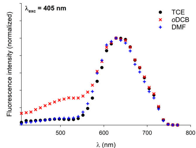
Figure 10. Normalized emission spectra of xerogels prepared by gel deposition of C_3Pyr/C_3NDI (1:1) mixtures in TCE, o DCB, and DMF for \lambda_{exc} = 405 nm.
