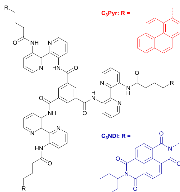
Scheme 1. Chemical structures of C_3\text{Pyr} and C_3\text{NDI}
