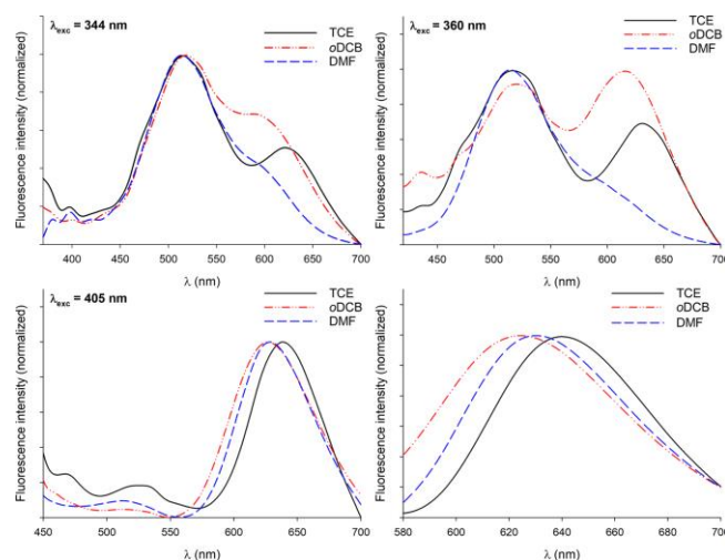
Figure 8. Normalized emission spectra of C 3 Pyr / C 3 NDI (1:1) organogels (C = CGC) upon excitation at different wavelengths (Bottom right corner: irradiations at \lambda_{\text{exc}} = 525 (TCE), 512 (oDCB) and 523 nm (DMF)).
