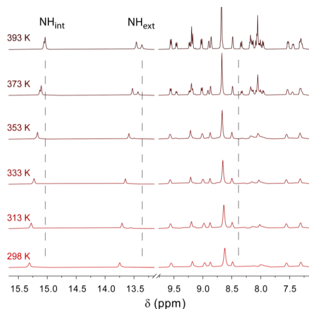
Figure 3. Variable temperature 1 H NMR spectroscopy of a C 3 Pyr/C 3 NDI (1/1) mixture in TCE-d 2 ([C 3 Pyr] = [C 3 NDI] = 5.2 mM)
