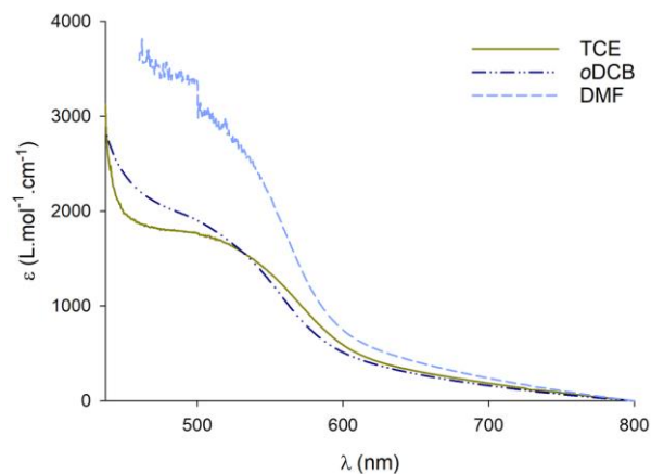
Figure 4. Top. Visible absorption spectra of the individual compounds C 3 Pyr (5.2 mM), C 3 NDI (5.2 mM) and their equimolar mixture C 3 Pyr/C 3 NDI ( C_T = 10.5 \text{ mM} ) in TCE. Bottom. Visible absorption spectra of C 3 Pyr/C 3 NDI (1:1) organogels in TCE, o DCB and DMF ( C_T = \text{CGC} )
