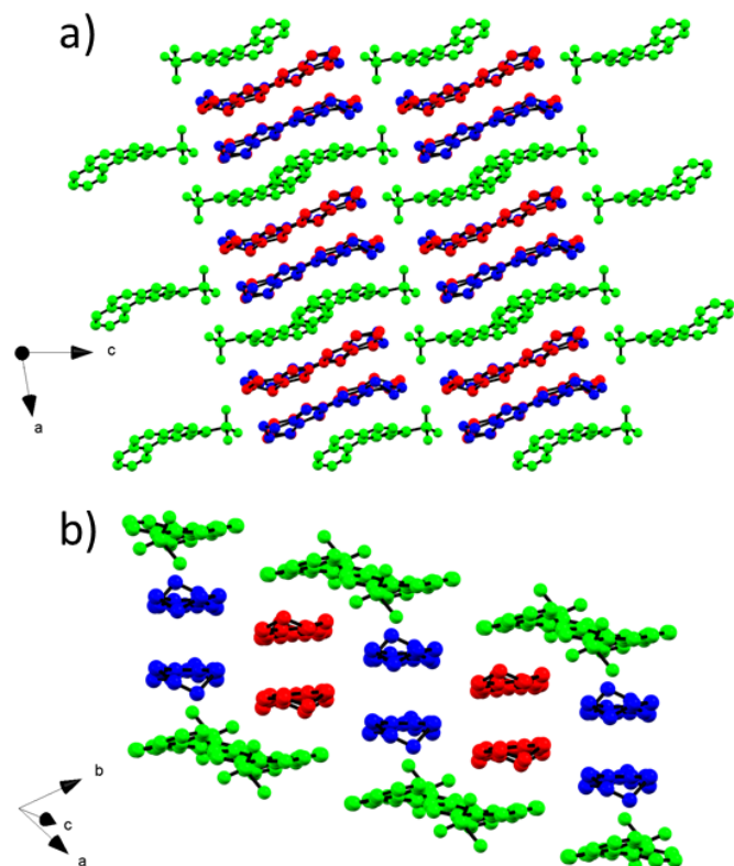
Figure 5. Crystal structure of (\text{BEDT-TTF})_2([\text{4}]\text{heliceneSO}_3) viewed a) along the b axis and b) perpendicularly to the dimer stacks (red : BEDTTTF B ; blue : BEDTTTF A ; green : [\text{4}]\text{heliceneSO}_3 ; solvent molecules and hydrogen atoms have been omitted for the sake of clarity).
