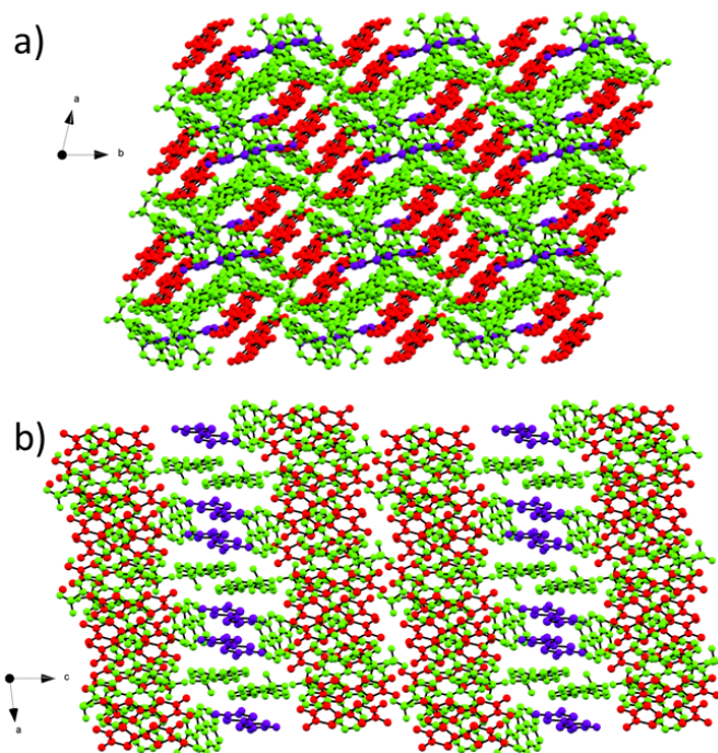
Figure 4. Crystal structure of (\text{TMTSF})_5([\text{4]heliceneSO}_3)_5 viewed along the a) c axis and b) b axis (red: TMTSF stacked by four; violet: TMTSF stacked by two; green: [4]helicene \text{SO}_3 , solvent and thionyl chloride molecules and hydrogen atoms have been omitted for the sake of clarity).
