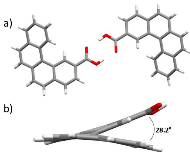
Figure 1. X-Ray structure of compound 2 with a view of a) the H-bonded dimer and b) the interplane angle of the helicenic scaffold (Carbon: grey; Oxygen: red; Hydrogen: white).
