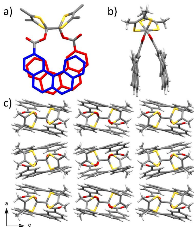
Figure 2. X-Ray structure of the adduct electrocrystallized from TMTTF and 2 with a) a front view of the adduct (the two helicene moieties are highlighted in blue and red), b) a side view of the adduct and c) packing along b (Carbon: grey; Oxygen: red; Sulfur: yellow; Hydrogen: white).
