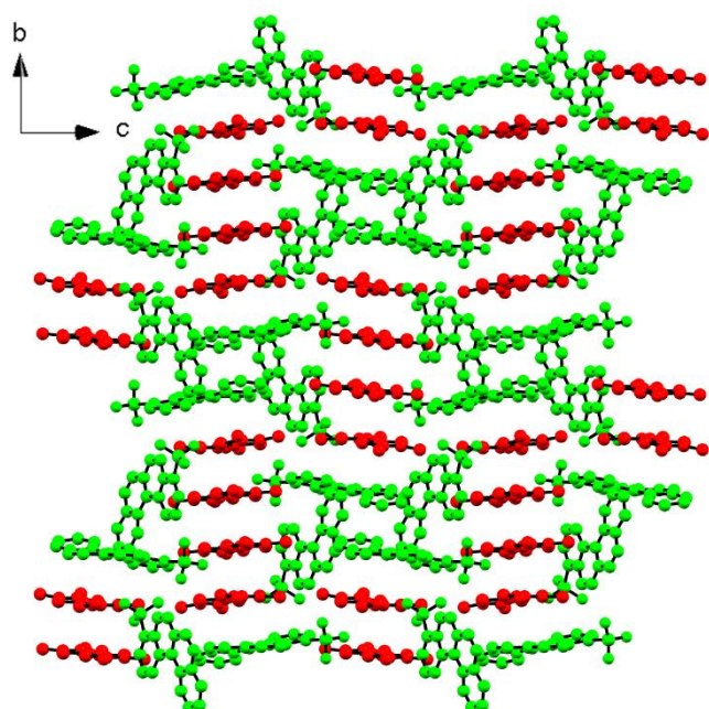
Figure 3. Crystal structure of (\text{TMTTF})_2([\text{4]heliceneSO}_3)_2 viewed along the a axis (red: TMTTF and green: [4]helicene \text{SO}_3 ).
