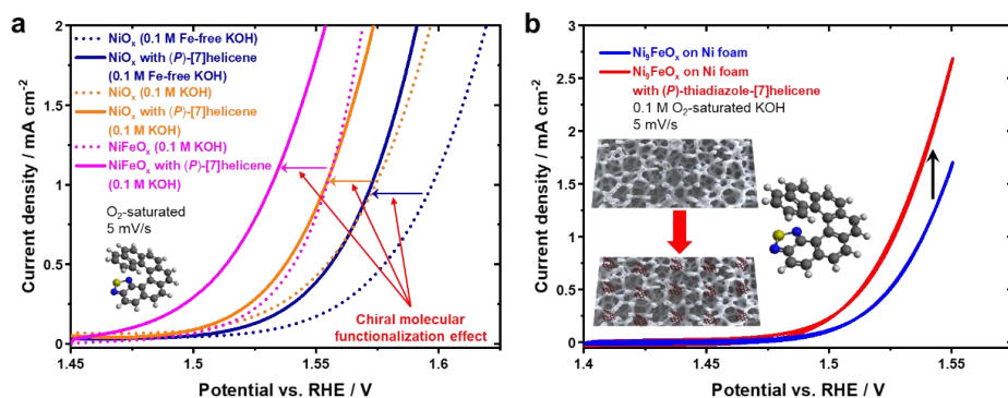
Fig. 2 | Comparison of chiral molecule effect with Fe-doping effect. a , chiral molecular functionalization enhancement on NiO x islands in Fe-free, NiO x islands in KOH (unpurified) and NiFeO x islands in KOH (unpurified). b , chiral molecular functionalization enhancement at Ni 9 FeO x deposited on Ni foam.
