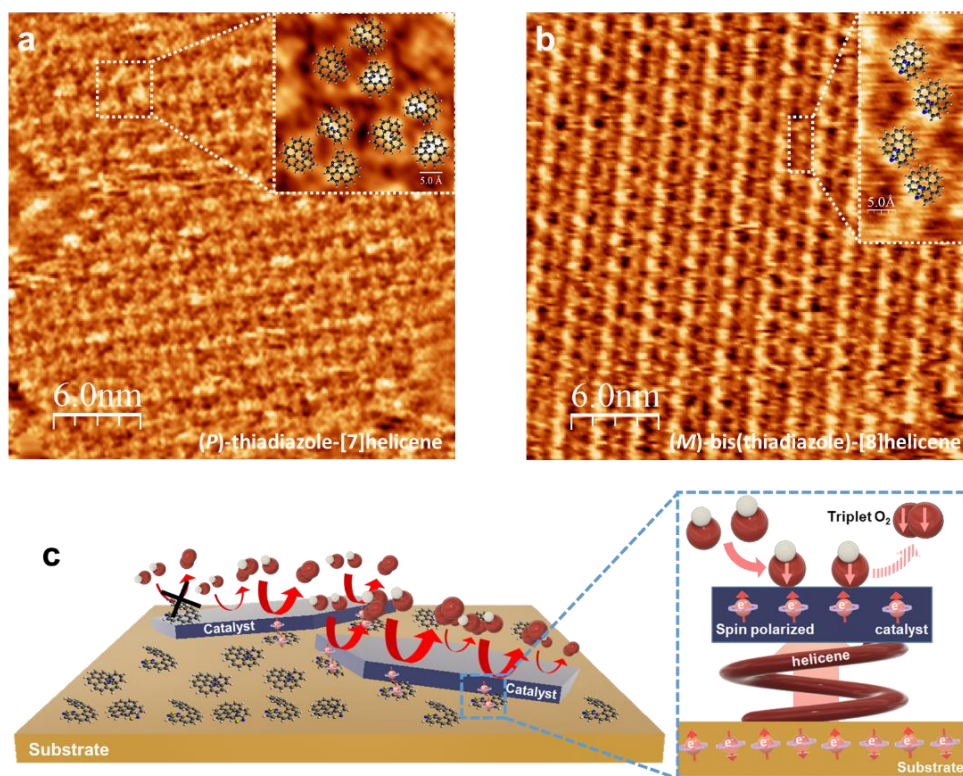
Fig. 4 | Helicene SAM and effect on the OER activity. a, an STM image of SAM of ( P )-thiadiazole-[7]helicene (image size: 30 \text{ nm} \times 30 \text{ nm} , tunneling current: 25 \text{ pA} , sample bias: -5 \text{ mV} ). The dashed square marks a trimer of the molecules. A high resolution image (image size: 2.2 \text{ nm} \times 2.2 \text{ nm} , tunneling current: 20 \text{ pA} , sample bias: 20 \text{ mV} ) showing one trimer is
