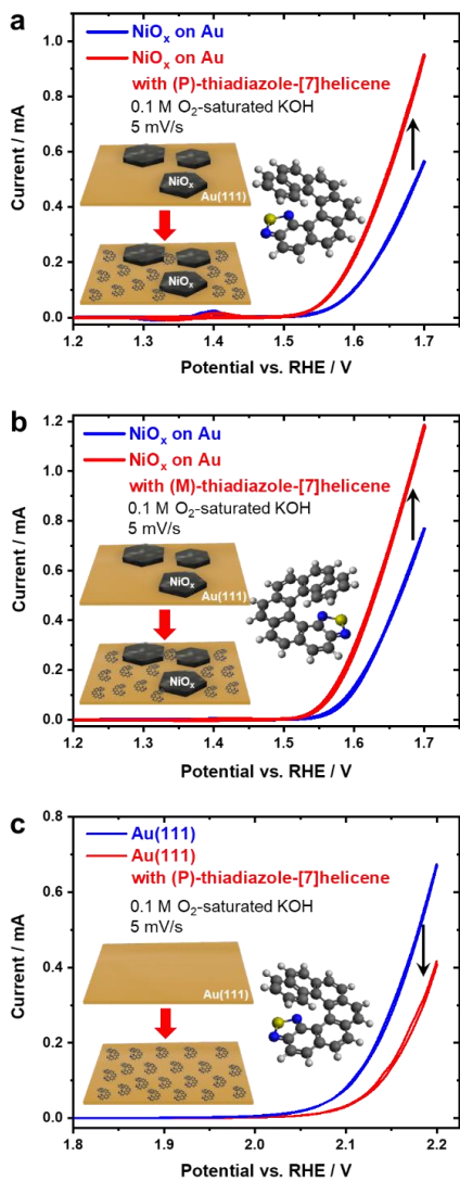
Fig. 1 | Helicene enantiomer functionalization effect on the OER activity. OER activity of a ( P )-thiadiazole-[7]helicene and b ( M )-thiadiazole-[7]helicene embedded NiO x electrodes in 0.1 M O 2 -saturated KOH.
