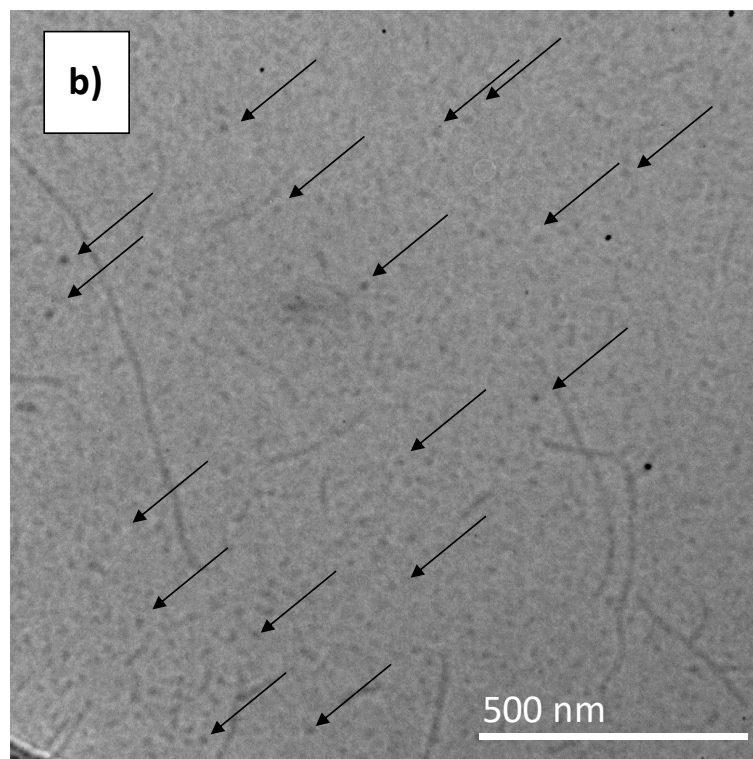
Figure 1. CryoTEM of particles formed by PEO-TTF-U 2 with the "DMSO-route" (water/DMSO = 99/1 v/v, C = 1 g.L -1 ) a) before oxidation, revealing long nanocylinders and a few nanospheres
