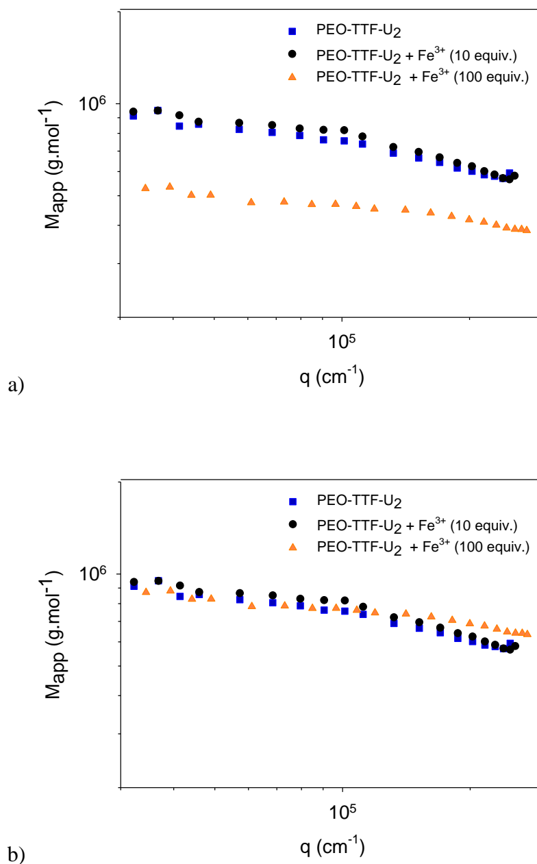
Figure 2. a) Angular dependency of the apparent molar mass of PEO-TTF- \text{U}_2 self-assemblies ( 0.5 \text{ g.L}^{-1} prepared via the "DMSO-route") in water/DMSO (99/1 v/v) before and after oxidation
