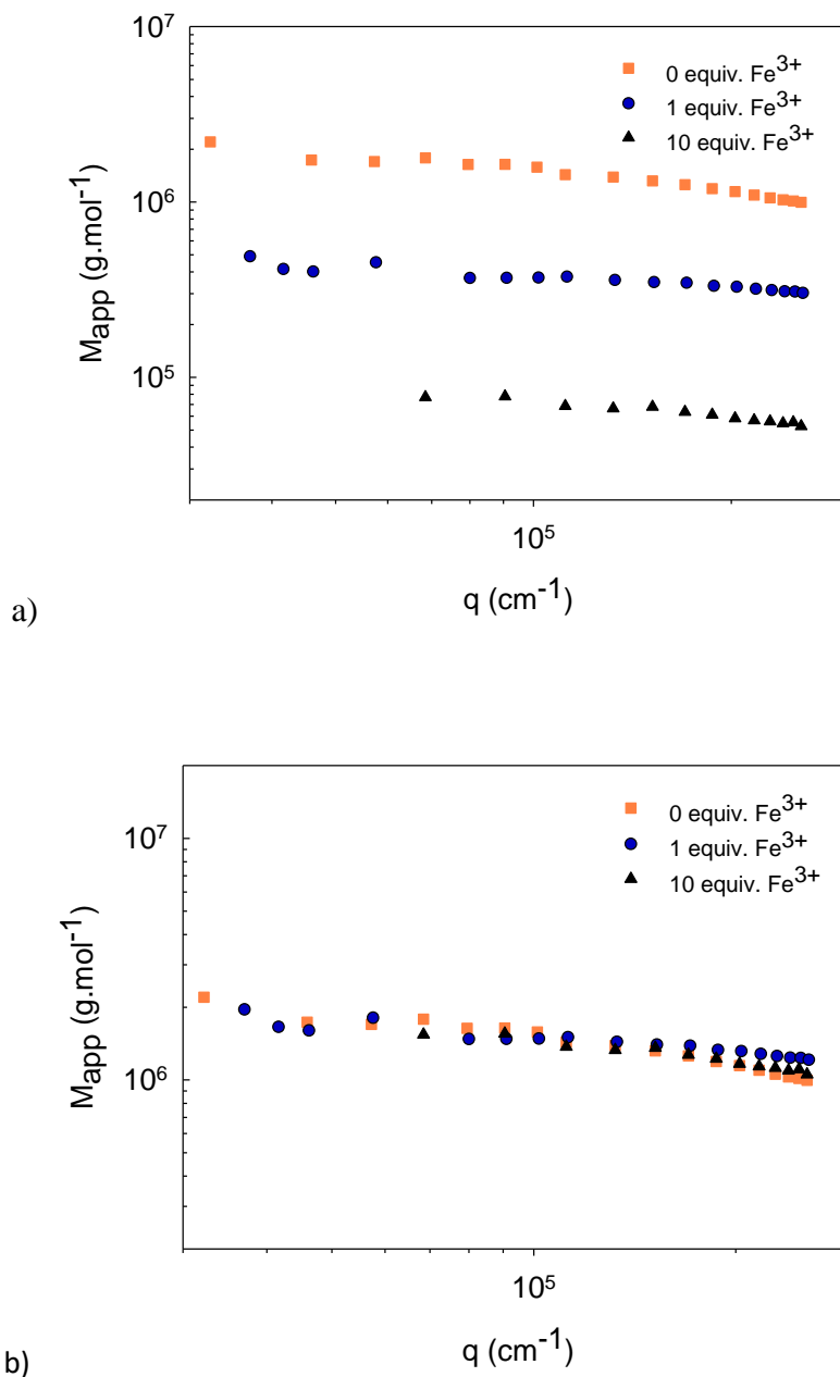
Figure 5. a) Angular dependency of the apparent molar mass of PEO-TTF-U 2 dispersions at C = 0.5 \text{ g.L}^{-1} in ACN (nanocylinders transferred from the water/DMSO 99/1 v/v solution, see SI
