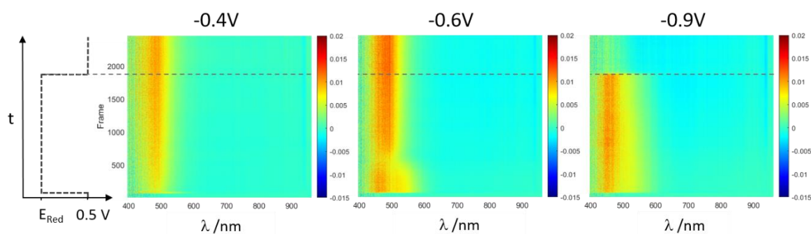
Figure 5. A-SEC over chronoamperometric experiments recorded on polycrystalline gold electrode in the presence of 1 \text{ mM} 4-NBD in atmospheric conditions for E_{\text{Red}} = -0.4 , -0.6 , and -0.9 \text{ V} . Potential program: 30 \text{ s} at +0.5 \text{ V} , 15 \text{ min} at E_{\text{Red}} , 5 \text{ min} at +0.5 \text{ V} .
