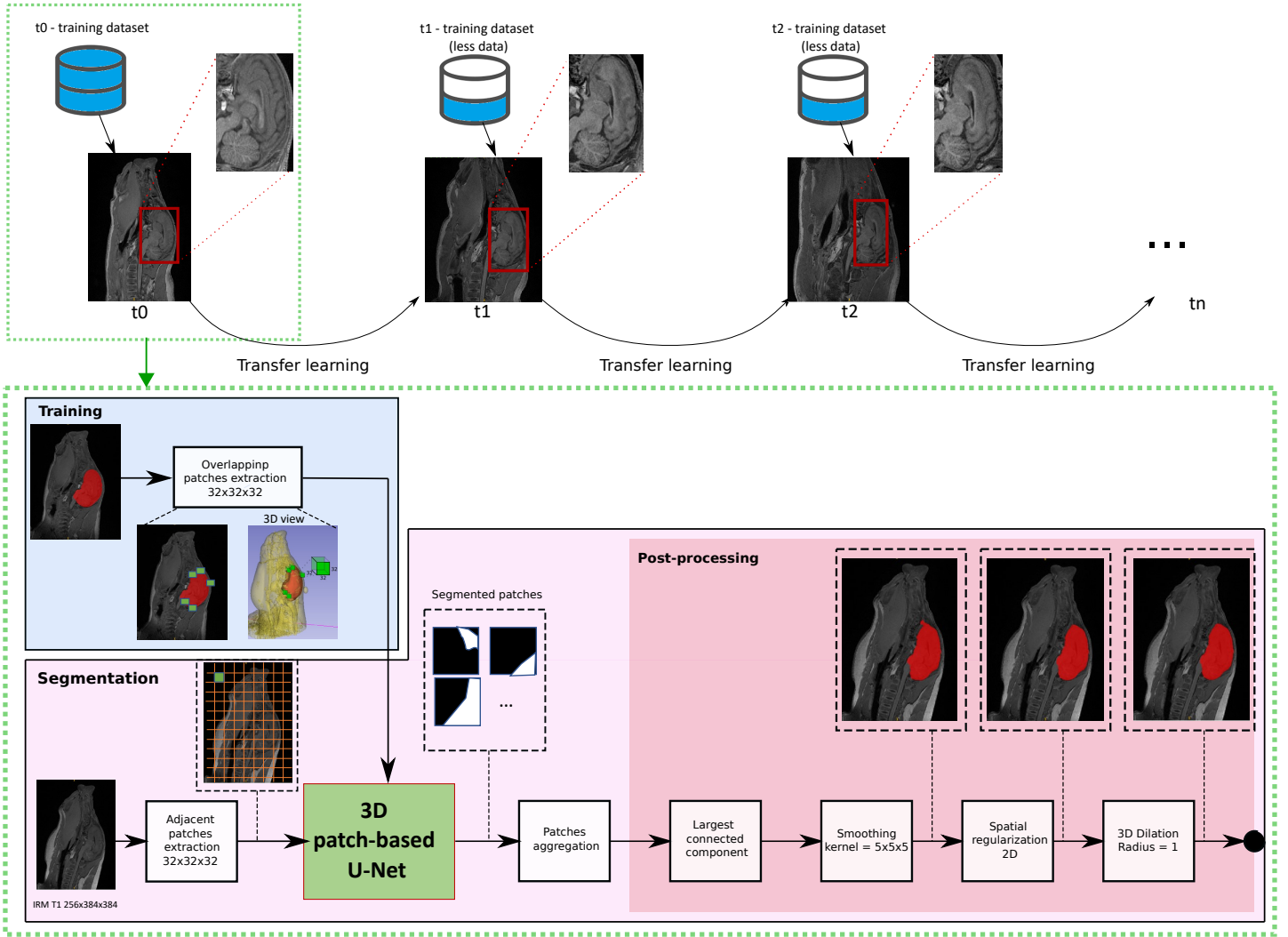
Figure 1: Overview of the proposed automatic piglet brain segmentation method on T1 MRI. The upper part illustrates the principle of transfer learning applied as the brain develops (intensification of contrasts, fat formation, growth). The lower part details the proposed segmentation pipeline (deep learning and post-processing).
