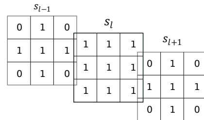
Figure 4: 3D Connectivity/Structuring element considered for connected component labelling/morphological dilation.
