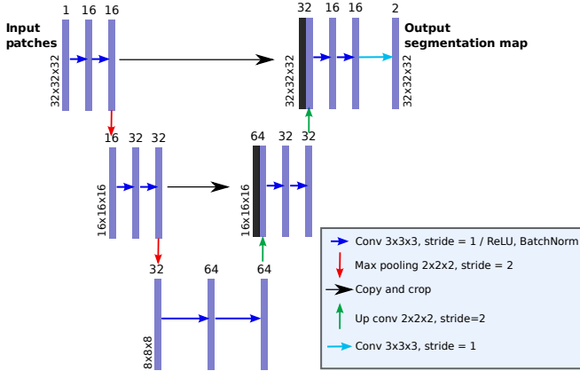
Figure 2: Architecture of the implemented U-Net
