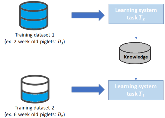
Figure 5: Transfer learning: illustrated principle ( s is relative to the source domain (in our case the young piglets) and t to the target domain (the older piglets))
