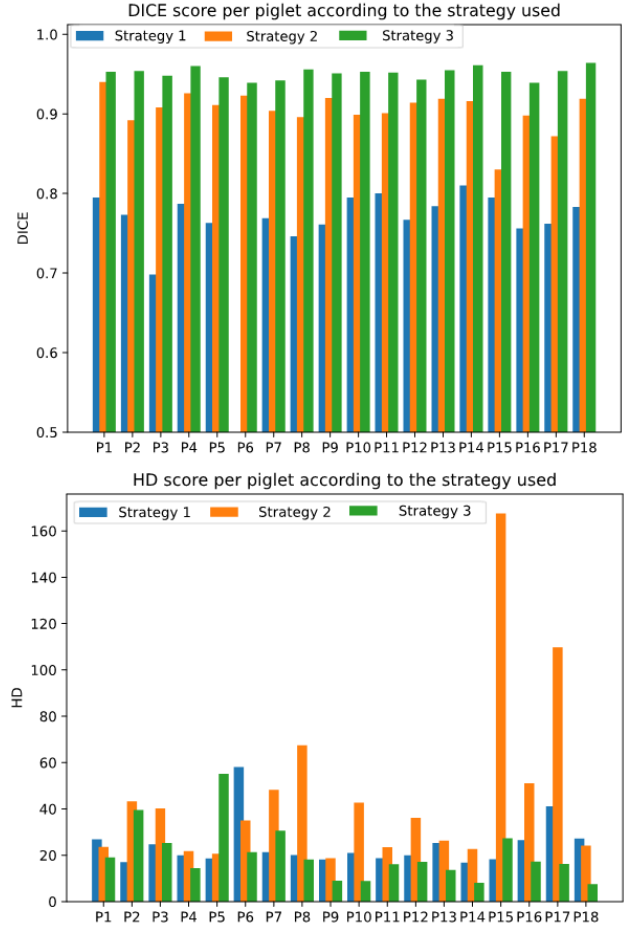
Figure 7: Detailed performance results (Dice and HD) obtained on the eighteen 2-weeks test piglets (P1 to P18) with the three strategies of training patches distribution.
