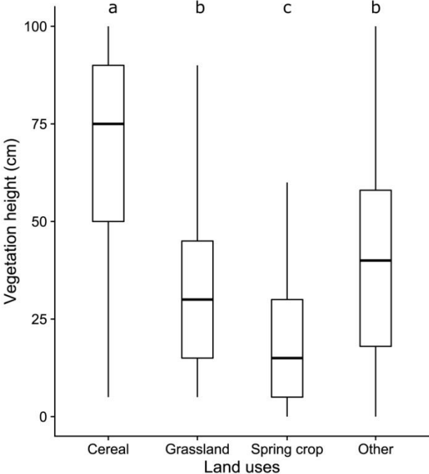
Fig. S2. Vegetation height (boxplot with median, lower and upper quartile, lowest and highest value) in relation to land use. Significance between land use differences in post hoc tests are indicated by different lowercase letters.
