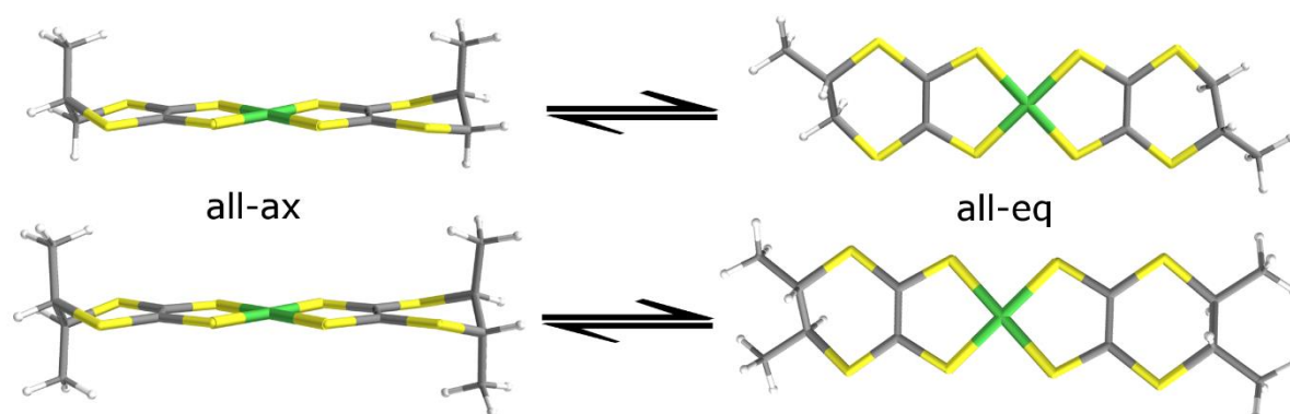
SCHEME 2 Conformational equilibrium in solution for [Ni(me-dddt) 2 ] -1/0 and [Ni(dm-dddt) 2 ] -1/0 . Only the (S) enantiomers are shown, and for [Ni(me-dddt) 2 ] only the trans isomer is represented.
