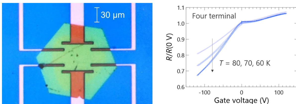
Fig. 9 Microscope image of the thin hexagonal crystal of [(S)\text{-}\mathbf{1}]_9(\text{Mo}_6\text{O}_{19})_5 \cdot (\text{CHBr}_3)_2 attached on the \text{SiO}_2/\text{Si} substrate with pre-patterned gold electrodes (left). Gate voltage dependence of normalized resistance of the crystal at selected temperatures of 60 K, 70 K, and 80 K (right).
