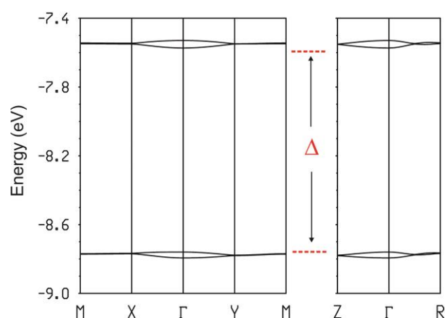
Fig. 11 Calculated three-dimensional band structure for the donor sublattice of [(rac)\text{-}\mathbf{1}]_2(\text{Mo}_6\text{O}_{19}) , where \Gamma = (0, 0, 0) , X = (a^*/2, 0, 0) , Y = (0, b^*/2, 0) , M = (a^*/2, b^*/2, 0) , Z = (0, 0, c^*/2) and R = (a^*/2, b^*/2, c^*/2) . \Delta is the energy gap between the filled and empty bands.
