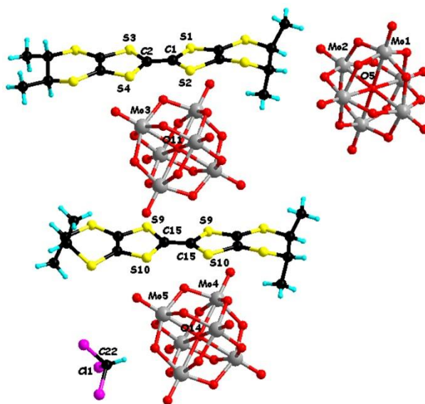
Fig. 1 Detail of the crystal structure of [(S)\text{-}\mathbf{1}]_9(\text{Mo}_6\text{O}_{19})_5 \cdot (\text{CHCl}_3)_2 with the two different donors (one and half independent), three different polyoxometallate dianions (two one third and one sixth independent) and a \text{CHCl}_3 solvent molecule (one third independent).
