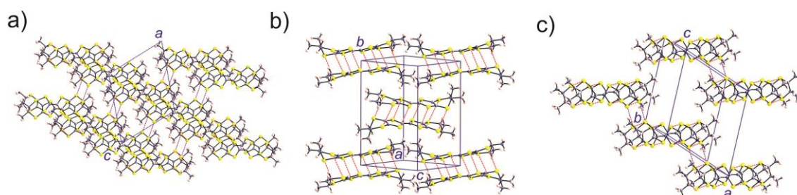
Fig. 10 Donor sublattice of the [(rac)\text{-}\mathbf{1}]_2(\text{Mo}_6\text{O}_{19}) salt. The \text{S}\cdots\text{S} contacts shorter than 3.9 \text{ \AA} are shown as dashed red (intra-dimer) and purple (inter-dimer) lines.
