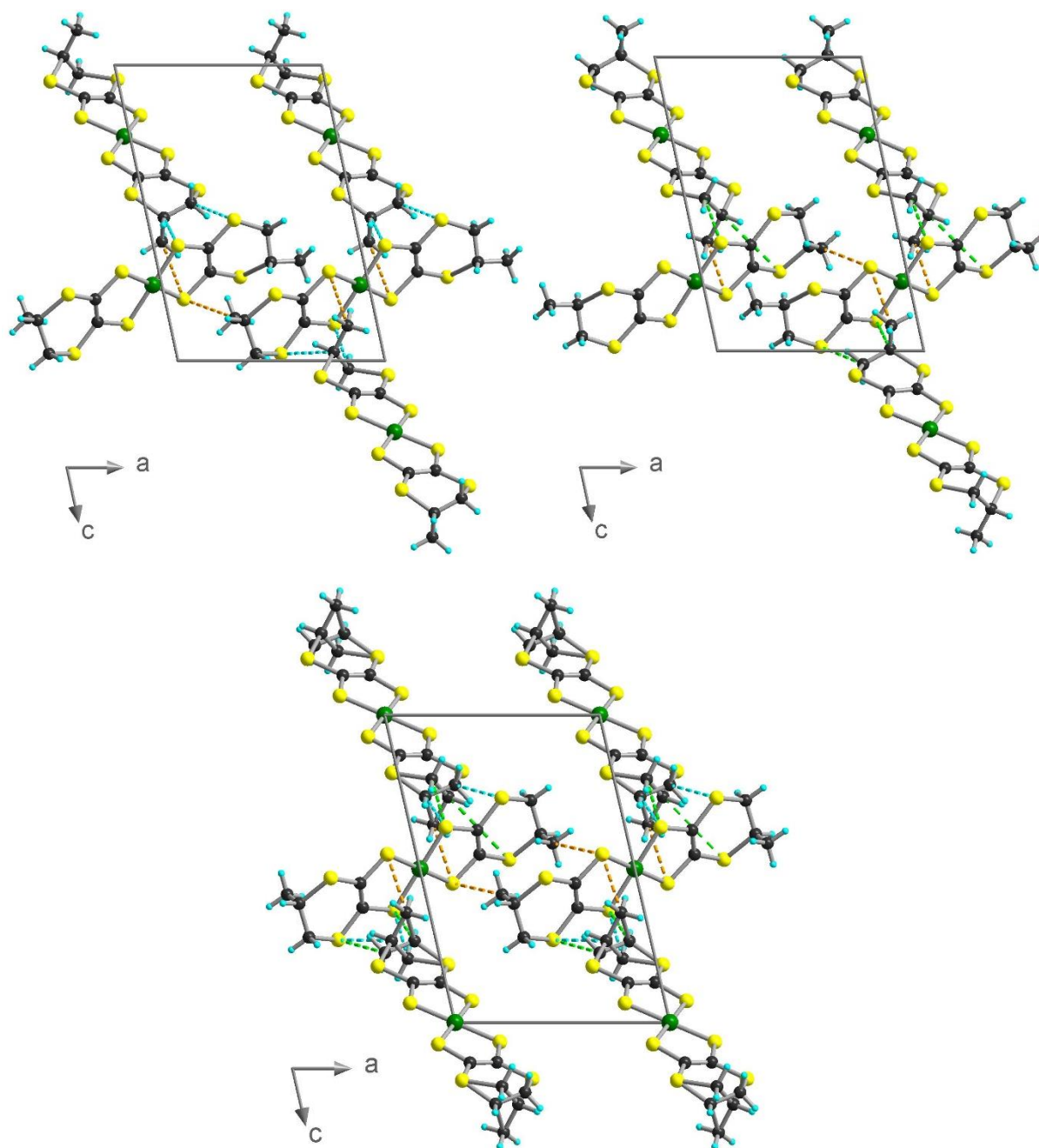
Fig. 3 Intermolecular C–H...S interactions (dashed lines) between the anionic complexes in (TBA)[Ni(S-me-dddt) 2 ] , (TBA)[Ni(R-me-dddt) 2 ] and (TBA)[Ni(S-me-dddt)(R-me-dddt)] . TBA cations are omitted for clarity. Color code: C (black), H (cyan), S (yellow), Ni (green). Cyan and light green dashed bonds correspond to the interactions involving S and R carbon atoms respectively, orange dashed bonds correspond to the methyl...S interactions which are present in both compounds.
