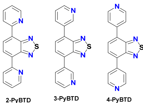
Scheme 1. 4,7-dipyridyl-BTD ligands used in the present study.
