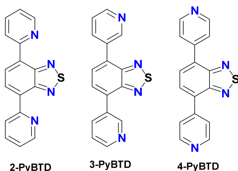
Scheme 1. 4,7-dipyridyl-BTB ligands used in the present study.
