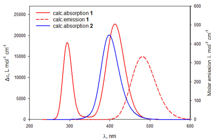
Figure 9. Calculated UV-Vis absorption (solid lines) and emission (dashed line) spectra of complexes 1 (red) and 2 (blue) with a gaussian broadening (FWHM = 3000\text{ cm}^{-1} ); TD-DFT / PBE1PBE / TZVP.
