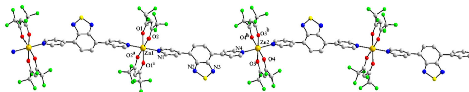
Figure 6. Linear chain in the crystal structure of compound 7 . Symmetry operation a = -x, 2-y, 2-z ; b = 2-x, -y, 1-z .
