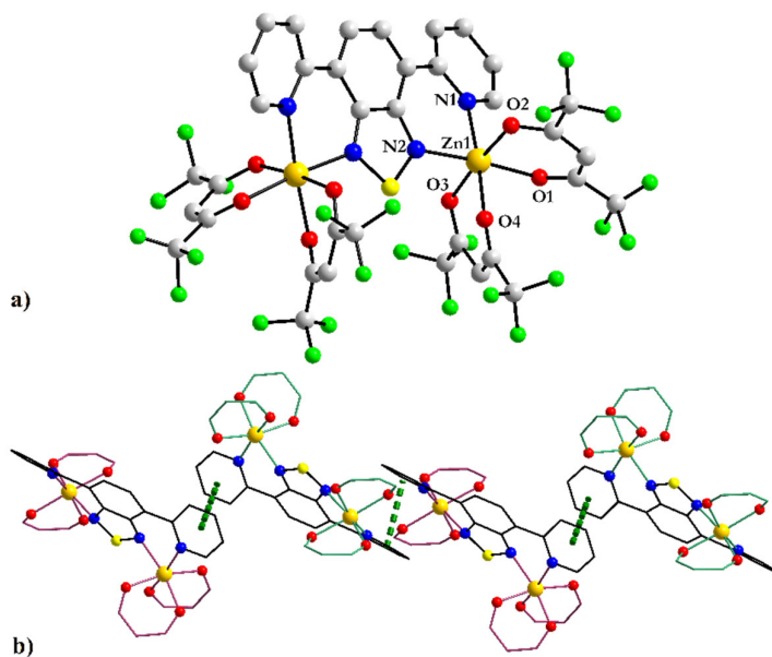
Figure 2. (a) Crystal structure of [Zn_2(hfac)_4(2-PyBTd)] ( 2 ) with a partial atom numbering scheme; (b) View of the packing diagram illustrating the opposite chirality of the metal centers from neighboring binuclear complexes (green— \Delta configuration, violet— \Lambda configuration) ( CF_3 groups have been omitted for clarity).
