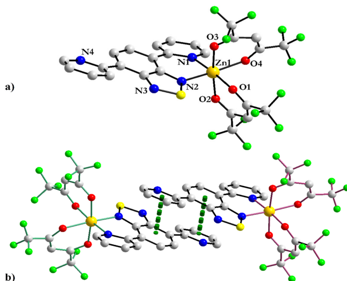
Figure 1. (a) Crystal structure of [Zn(hfac)_2(2-PyBTD)] ( 1 ) with a focus on the coordination sphere of Zn^{II} and partial atom numbering scheme; (b) Supramolecular dimer built out of mononuclear units of opposite chirality (green— \Delta configuration, violet— \Lambda configuration) through \pi – \pi stacking interactions.
