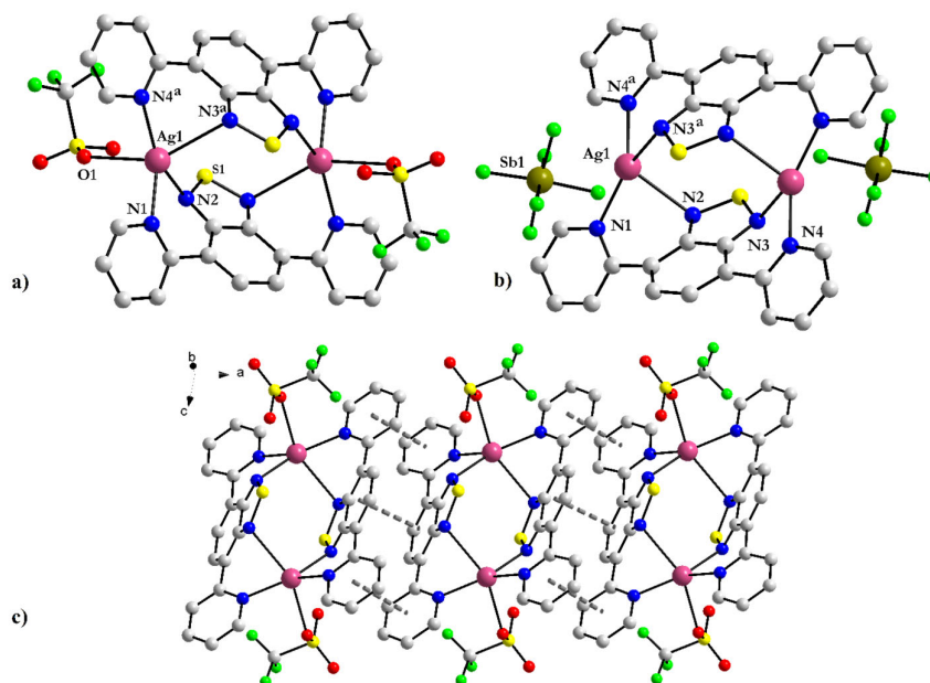
Figure 3. (a) Crystal structure of complex [\text{Ag}(\text{CF}_3\text{SO}_3)(2\text{-PyBTD})]_2 3 . Symmetry operation ^a = 1-x, 1-y, 1-z ; (b) Crystal structure of complex 4 . Symmetry operation ^a = 1-x, -y, 1-z ; (c) View of a one-dimensional assembly in compound 3 highlighting the \pi - \pi stacking interactions between neighboring binuclear species.
