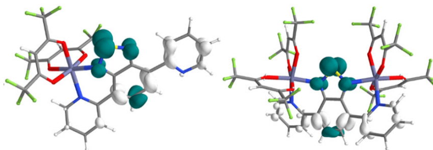
Figure 10. Representation of the Electron Density Differences (EDD) for the S_1-S_0 transition of complex 1 (left) and the S_5-S_0 transition of complex 2 (right). The excited electron and hole regions are indicated by, respectively, blue and white surfaces.
