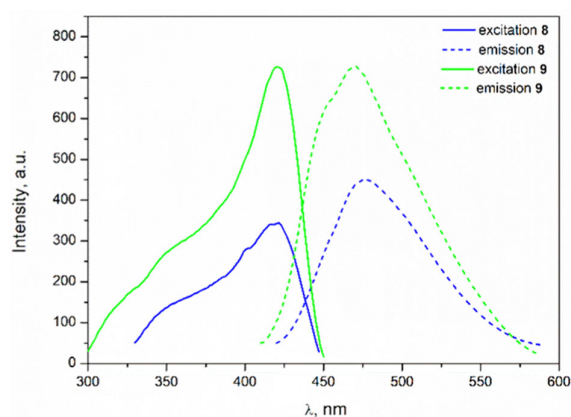
Figure 12. Emission (dotted curves, \lambda_{ex} = 410 nm for 8 and \lambda_{ex} = 400 nm for 9 ) and excitation (solid curves, \lambda_{em} = 475 nm for 8 and \lambda_{em} = 470 nm for 9 ) for complexes 8 (blue) and 9 (green).
