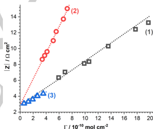
Fig. 2 Absolute values of impedance ( |Z| ) at 10 \text{ kHz} vs. surface coverage for (1) NB, (2) AQ and (3) PhFc layers for 1 min – 90 min grafting times. NB layers were grafted from a 0.1 \text{ mM} solution of NBD compound. The AQ and PhFc layers were grafted from the 1 \text{ mM} solutions of the corresponding amine derivatives with in-situ generation of diazonium salts. The resistance of electrolyte was subtracted from |Z| . The dotted lines represent the fit with linear least squares.
