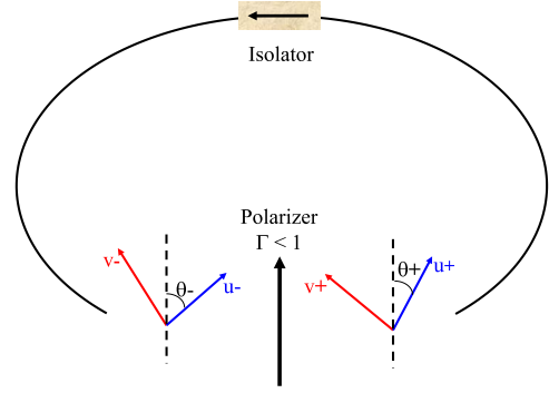
FIG. 6. (Color online) Orientation angles \theta_- and \theta_+ .
