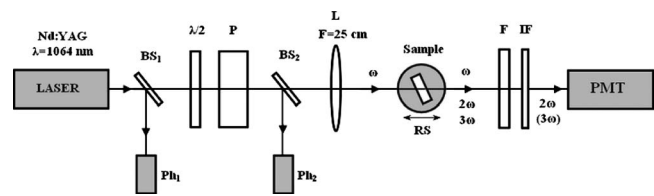
FIG. 1. Experimental setup for SHG and THG measurements: the beam splitters ( BS_1 , BS_2 ), the synchronization and control photodiodes ( Ph_1 , Ph_2 ), ( \lambda/2 ), the Glan polarizer, the converging lens, RS, the filters, IF, and PMT.
