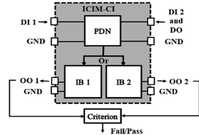
Fig. 1. Dual port ICIM-CI model structure of an IC (Airrieau et al., 2016).
