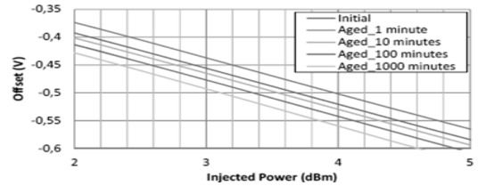
Fig. 17. Ageing impact on the DC offset voltage as a function of the RF power at 200 MHz (Huang et al., 2015).
