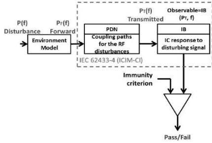
Fig. 14. Block diagram for the ICIM-CI model with integrated external environmental model for ageing (Dubois et al., 2015).
