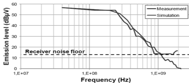
Fig. 13. Simulated and measured conducted EM emission level from the digital core (Boyer et al., 2013a).
