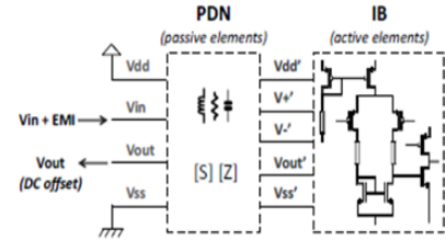
Fig. 16. Proposed ageing-aware EM susceptibility model structure of the operational amplifier (Huang et al., 2015).
