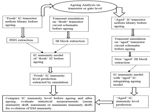
Fig. 15. Proposed ageing-aware ICIM model methodology.
