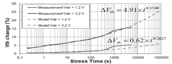
Fig. 18. Threshold voltage variations depending on the different ageing conditions (Boyer et al., 2013b).
