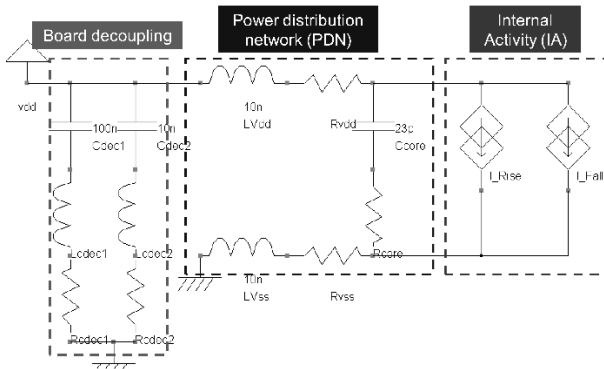
Fig. 11. Emission model structure for the digital core circuit embedded in the IC (Boyer et al., 2013a).
