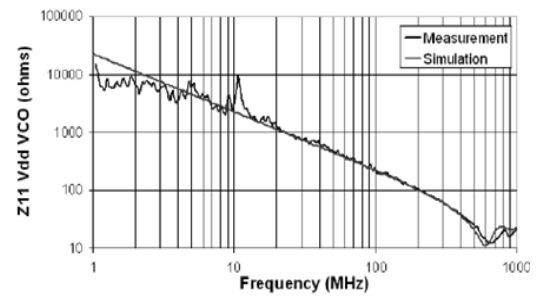
Fig. 9. Impedance measurement from VDD VCO pin (Boyer et al., 2012).
