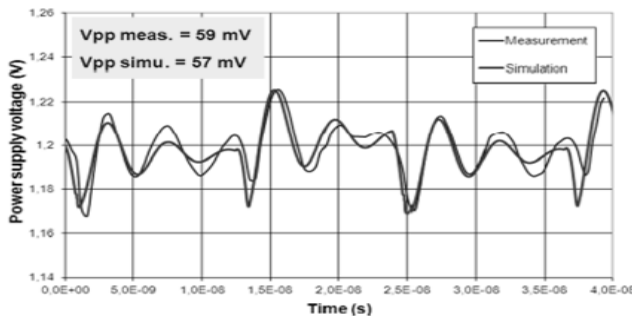
Fig. 12. Simulated and measured digital core power supply voltage fluctuation (Boyer et al., 2013a).
