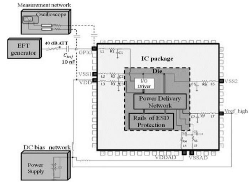
Fig. 3. IC model structure with EFT setup (Zhang et al., 2014).
