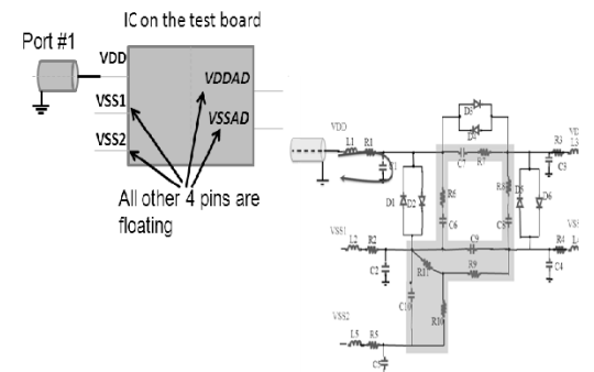
Fig. 7. Measurement method for IC package model extraction (Zhang et al., 2010).
