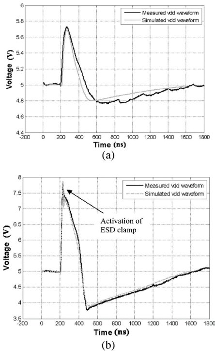
Fig. 8. Model validation result (a) EFT voltage 200V (b) EFT voltage 1600 V applied to the VDD pin (Zhang et al., 2014).
