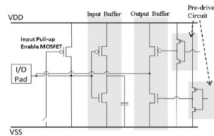
Fig. 4. IC model structure with EFT setup (Zhang et al., 2014).
