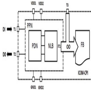
Fig. 2. Structure of the proposed ICIM-CPI model (Durier and Fernandez-Lopez, 2018).
