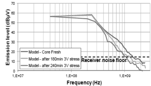
Fig. 19. Evolution of the EM emission level of the digital core circuit due to ageing stress (Boyer et al., 2014).
