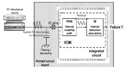
Fig. 5. IC immunity model for the PLL component including the DPI test setup (Boyer et al., 2012).
