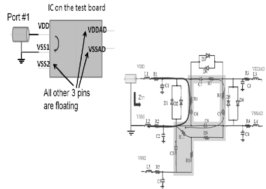
Fig. 6. Measurement method for the IC PDN model extraction (Zhang et al., 2010).
