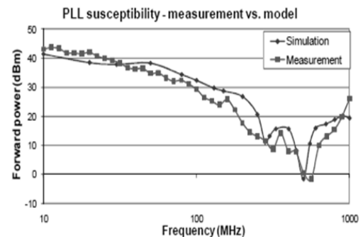
Fig. 10. Immunity profile comparison between the model and measurements (Boyer et al., 2012).
