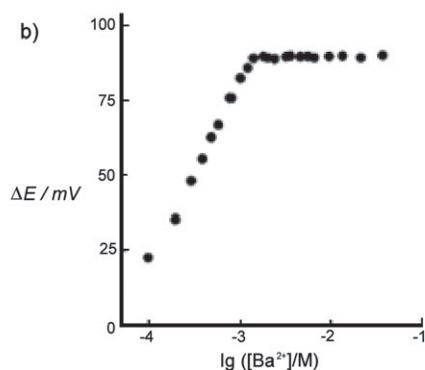
Fig. 7 (a) A dendrimer persubstituted with a redox-responsive ligand; (b) plot of \Delta E (= E_{\text{pa1}}([\text{Ba}^{2+}] = 0) - E_{\text{pa1}}([\text{Ba}^{2+}] \neq 0)) vs. \log([\text{Ba}^{2+}]) for dendrimer modified Pt electrodes (ref. 61). Copyright Wiley-VCH Verlag GmbH & Co. KGaA. Reproduced with permission).
