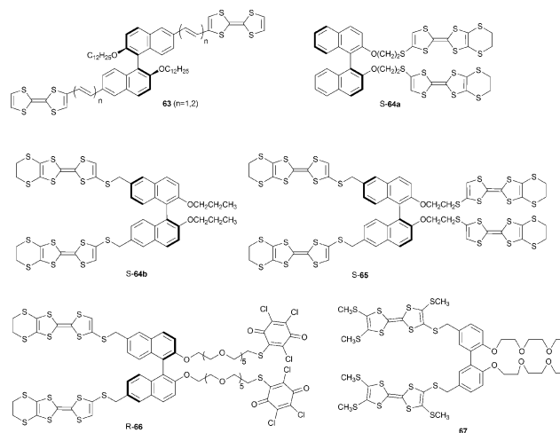
Scheme 29 C 2 -Symmetric TTF-based assemblies.
