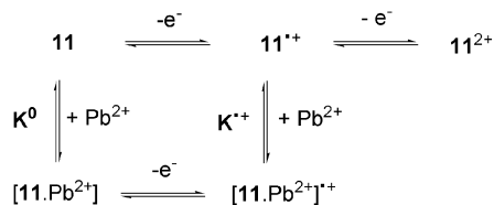
Scheme 4 Square scheme for the electrochemical titration of 11 with \text{Pb}(\text{ClO}_4)_2 .
