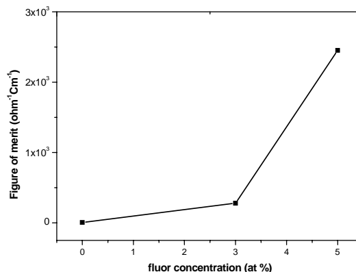
Fig. 4. Variation of figure of merit with fluorine dopant concentration of sprayed F- \text{In}_2\text{O}_3 films deposited at 450^\circ \text{C}
