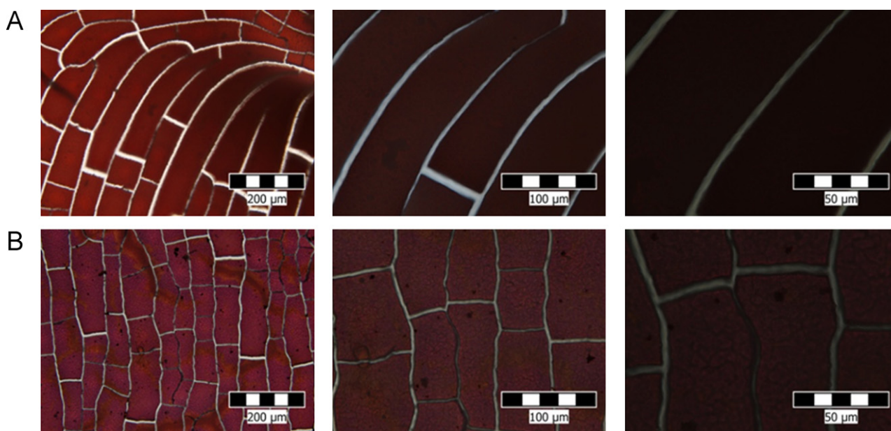
Fig. 5. Optical microscope images at various magnifications; from left to right: 20 \times ; 50 \times ; 100 \times for: (a) ST-HEMA impregnated with PDI 1; (b) ST-HEMA impregnated with PDI 2.
