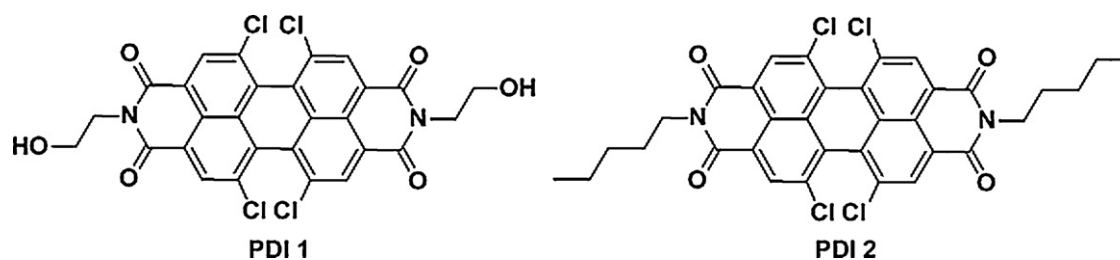
Scheme 1. The structures of the chromophores N,N' -bis(2'-hydroxyethyl)-1,6,7,12-tetrachloroerylene-3,4:9,10-bis(dicarboximide) (PDI 1) and N,N' -dipentyl-1,6,7,12-tetrachloroerylene-3,4:9,10-bis-(dicarboximide) (PDI 2).
