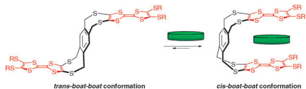
Fig. 35 Equilibrium between the trans boat-boat conformation (among other conformations) of 42 , and the closed cis boat-boat conformation suitable for sandwiching electron-poor aromatic guests.
