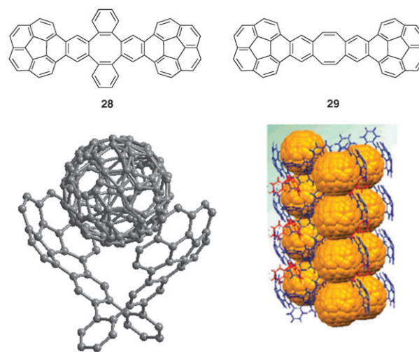
Fig. 24 X-Ray crystal structure of \text{C}_{60} @ 28 and corresponding crystal packing pattern (reproduced with permission from ref. 40. Copyright American Chemical Society 2010).
