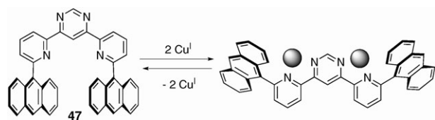
Fig. 39 Cation-driven two-stage U (left)/W (right) molecular shape switching.
