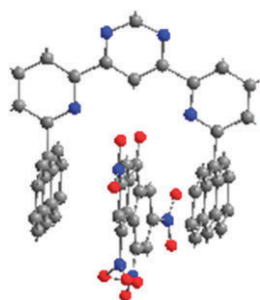
Fig. 40 X-Ray crystal structure of the complex 47 ·TNF.
