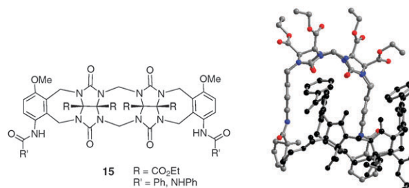
Fig. 8 Dimeric glycoluril molecular clip 15 and its self-association observed by X-ray study.
