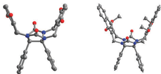
Fig. 5 X-Ray structures of diphenylglycoluril molecular clips 7d (left) and 8 (right).
