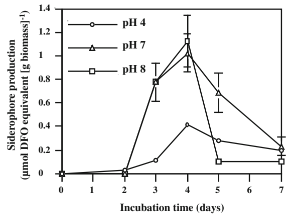
Fig. 2 Study of the kinetics of siderophore production by R. arrhizus in a commercial iron-depleted basal liquid medium buffered at pH 4 (circle), 7 (triangle) or 8 (square). Data are means of triplicate experiments. Bars indicate standard deviations. p < 0.01 for pH 7 and 8 versus pH 4 by Student's t test
