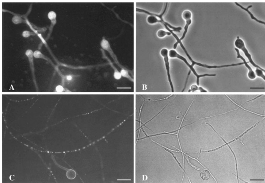
Fig. 5 Fluorescence (a and c) and phase-contrast (b and d) microscopies of R. arrhizus cells incubated with 10 \mu M NBD-DFO for 3 h (a and b) or 24 h (c and d). Mother cells of germ tubes presented a bright and uniform fluorescence after a
