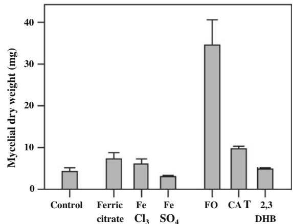
Fig. 3 Effect of various mineral and organic iron sources, feroxamine B (FO), catecholate (CAT) and 2,3-dihydroxybenzoate (2,3-DHB), on the growth of R. arrhizus . Data are means of triplicate experiments. Bars indicate standard deviations. p < 0.01 for FO versus other iron sources by Student's t test
