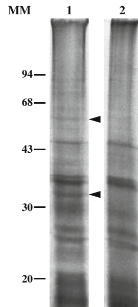
Fig. 4 SDS-PAGE analysis under reducing conditions of cytosolic extracts from R. arrhizus . The fungus was grown for 7 days at 37 °C on BLM + 1 mM iron citrate (lane 1) or + 1 \mu\text{M} FO (lane 2). Separated proteins were stained with Coomassie brilliant blue R 250, and their molecular masses were determined from the migration of standard proteins mentioned in kDa. Arrows indicate differences in protein patterns
