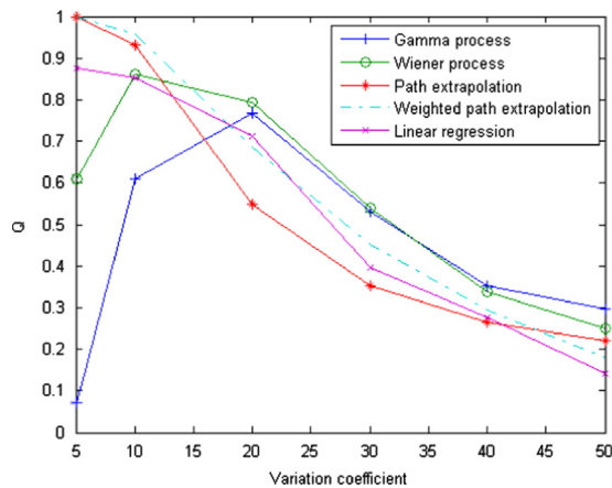
Fig. 11. Evolution of Q values with the variation coefficient.
