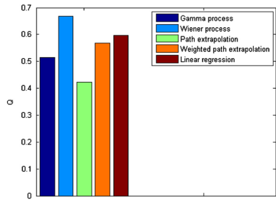
Fig. 7. Mean Q values for data generated by the Wiener process.
