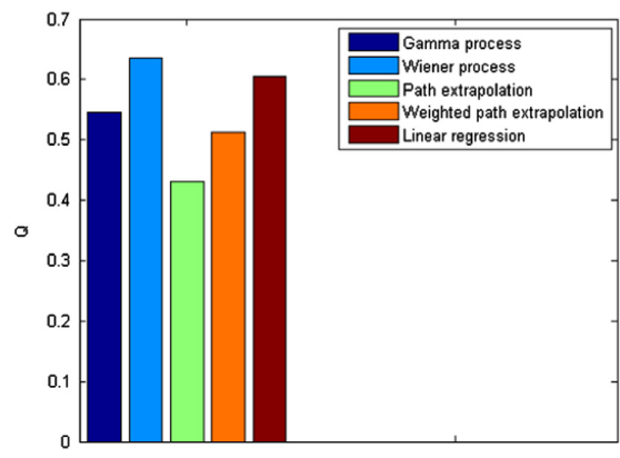
Fig. 6. Mean Q values for data generated by the gamma process.
