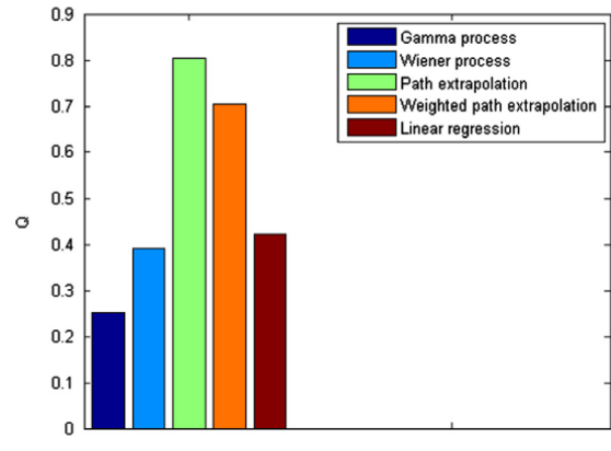
Fig. 8. Mean Q values for data generated by the linear path model.
