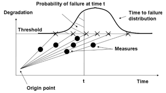
Fig. 3. Linear path extrapolation method.
