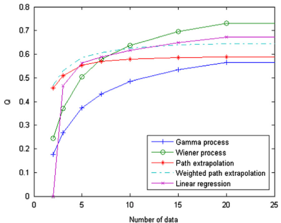
Fig. 9. Evolution of Q values with the number of data.
