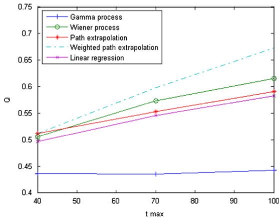
Fig. 10. Evolution of Q values with the time censorship.
