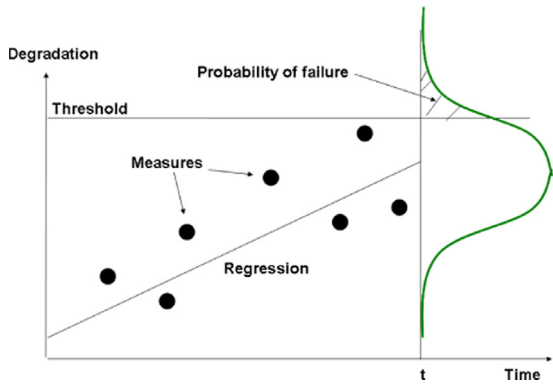
Fig. 4. Linear regression method.
