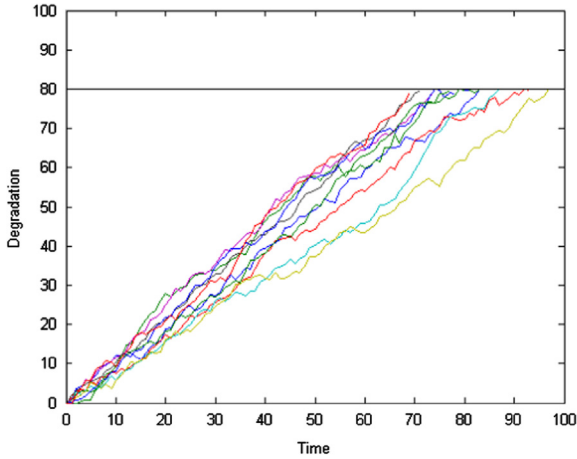
Fig. 2. Ten simulated Wiener process sample paths.
