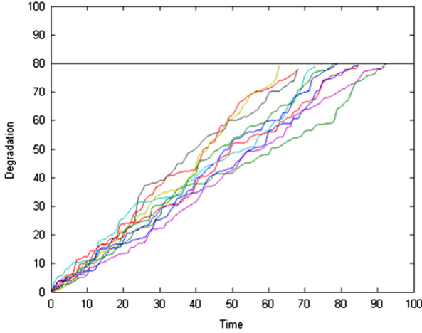
Fig. 1. Ten simulated gamma process sample paths.
