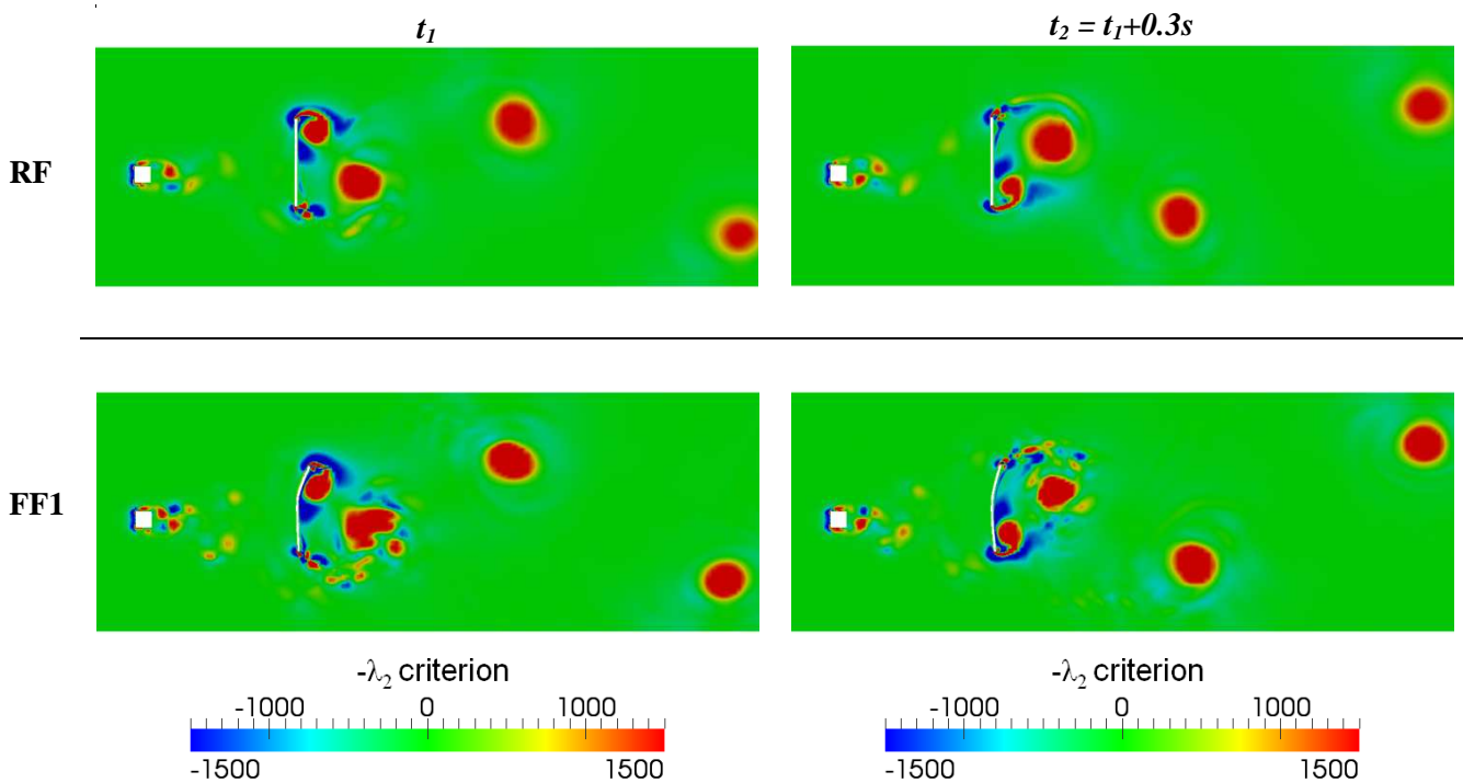
FIG. 2 - Snapshots of -\lambda_2 criterion for RF case (top figures) and FF1 (bottom figures) – Time step t_1 (left figures) has been arbitrary set and t_2 = t_1 + 0.3s (right figures)
