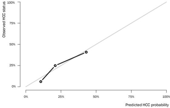
D1. Calibration plot: Random survival forest
