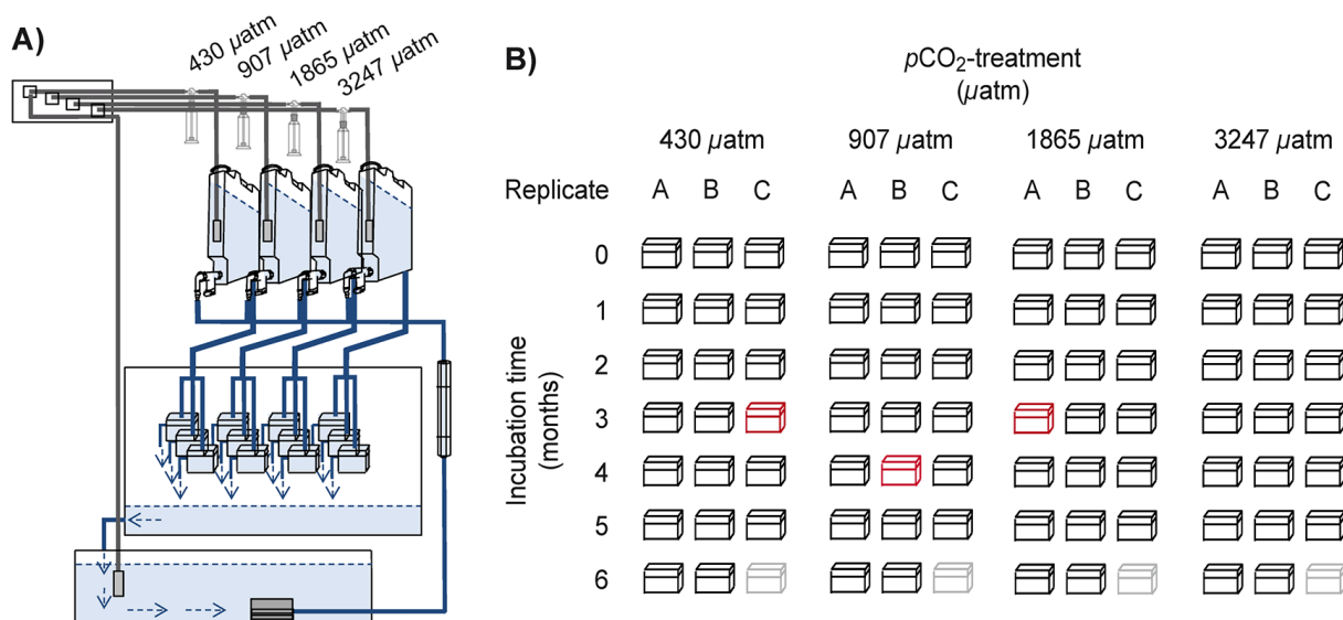
Fig. 1. (A) Scheme: experimental setup of A. aomoriensis in a closed flow-through system. Water equilibrated with four p\text{CO}_2 levels (430, 907, 1865 and 3247 \mu\text{atm} ) supplied from the compact jerrycans into the three replicated culture vessels and drained into a catchment tank, from where it was pumped up again to the jerrycans. (B) Experimental design: altogether 84 culture vessels, replication for four p\text{CO}_2 treatments (430, 907, 1865 and 3247 \mu\text{atm} ) during 6 months of incubation time. Red culture vessels: disappeared during incubation time. Culture vessels marked in light grey refer to treatments where carbonate chemistry parameters were measured in the supernatant seawater and sediment pore water in one of the three replicates after 6 months of incubation time.
