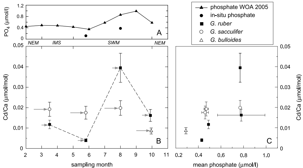
Figure 2. (a) Seawater phosphate concentration for the uppermost 75 m of the water column at 16^{\circ}\text{N} and 60^{\circ}\text{E} , derived from Garcia et al. [2006] (triangles) and seawater phosphate concentrations determined at the time of sampling (circles). (b) Cd/Ca ratios of live G. ruber (squares) and G. sacculifer (circles) collected in the Arabian Sea versus the sampling month. The arrows denote the life span (calcification period) of the two species, which is a fortnight for G. ruber and a full synodic lunar cycle for G. sacculifer . The different monsoon seasons are indicated in the upper part of Figure 2b. Also shown are data for the single in situ G. bulloides sample (triangle) from the North Atlantic. (c) Cd/Ca ratios of live G. ruber (squares), G. sacculifer (open circles), and G. bulloides (open triangles) versus mean seawater phosphate concentration for the upper 75 m of the water column. The horizontal error bars denote the range of seawater phosphate concentration that prevailed during the lifespan of the foraminifers. The uncertainty of the Cd/Ca data is given by the relative standard deviation (RSD) value of \pm 18\% obtained for multiple analyses of G. ruber tests of category B (see section 4.3 and Table 7).
