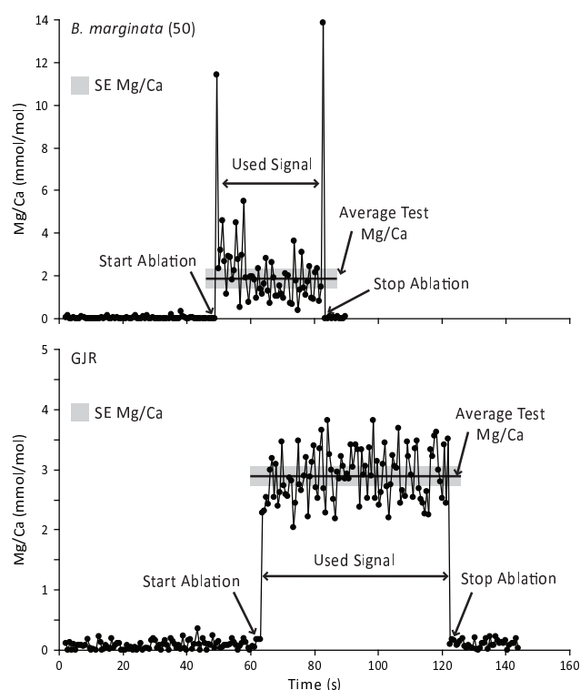
Fig. 1. Laser ablation profiles for Mg/Ca measured on benthic foraminifer B. marginata (upper panel) and the in-house GJR (Reichert et al., 2003) standard (lower panel). Parts of the profiles with elevated magnesium at the surface of the chamber walls are removed before calculating the average Mg/Ca. The absence of peak values for Mg/Ca in the GJR standard at the start and end of the ablation rule out any instrumental cause for the spikes observed in B. marginata .
