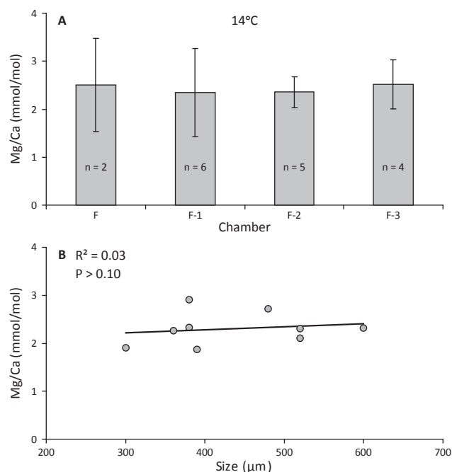
Fig. 3. Mg/Ca versus size for experiment 8 (14 °C). The upper panel depicts the average Mg/Ca value per measured chamber and the number of individual chambers analyzed ( n ). The final chamber is indicated by F and counted down in the whorl afterwards (F-1, F-2, etc.). Measured Mg/Ca values are statistically not different from one another. The lower panel displays the average Mg/Ca values of individual B. marginata born in the experiment versus their size. No trend can be observed between size and Mg/Ca.
