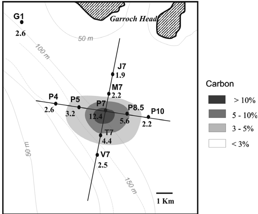
Fig. 4. Distribution of organic carbon in the surficial sediment (%d.w.).
