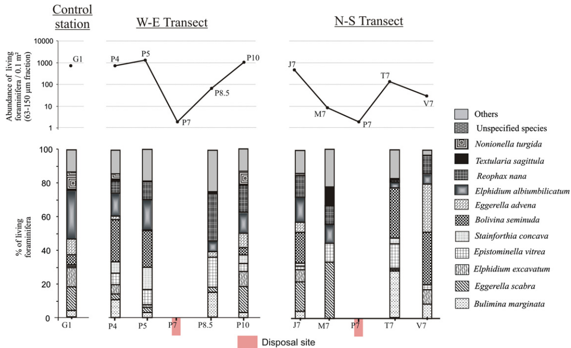
Fig. 8. Density and composition of the foraminiferal faunas (63–150 \mu\text{m} fraction) for 0.1 \text{m}^2 sediment surface.
