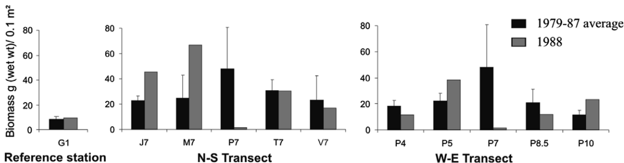
Fig. 13. Comparison of macrofaunal biomass in 1988 with the average value of the 1979–1987 period.
