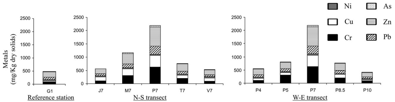
Fig. 6. Distribution of heavy metals in the sediments along the transects.
