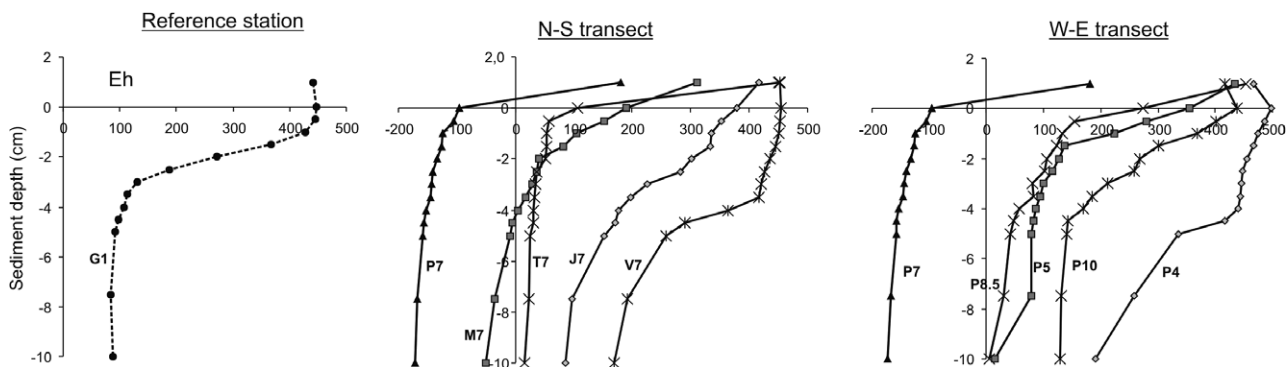
Fig. 2b. Profiles of redox potential in the sediment until 10 cm depth.
