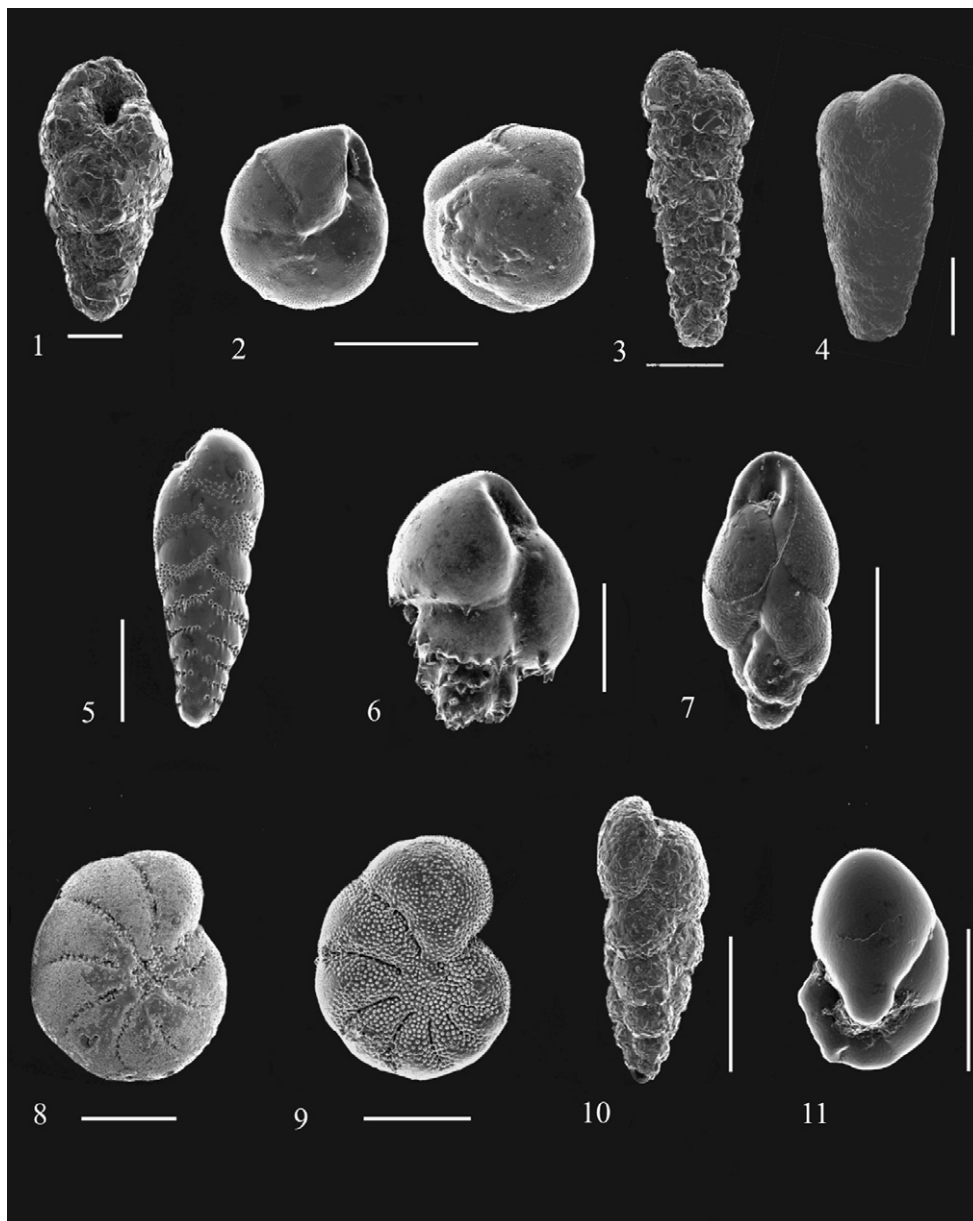
Plate 1. SEM images of the dominant foraminiferal taxa (1, Eggerella scabra ; 2, Epistominella vitrea ; 3, Textularia porrecta ; 4, Textularia sagittula ; 5, Bolivina seminuda ; 6, Bulimina marginata ; 7, Stainforthia concava ; 8, Elphidium excavatum ; 9, Elphidium albumbilicatum ; 10, Eggerella advena ; 11, Nonionella turgida ). Scale bar = 100 \mu\text{m} .
