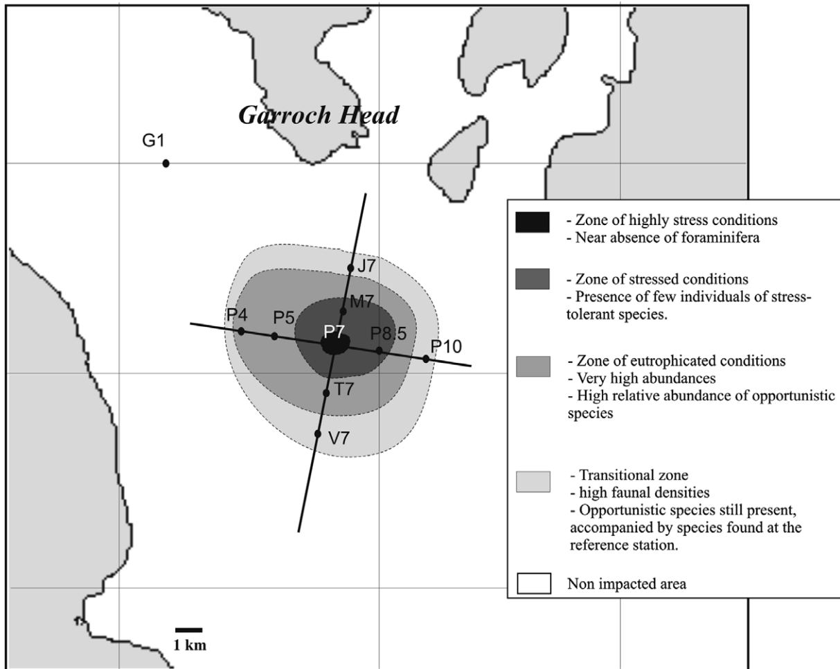
Fig. 18. Overview map, indicating the succession of foraminiferal zones with decreasing environmental impact at increasing distance from the sewage sludge disposal site.
