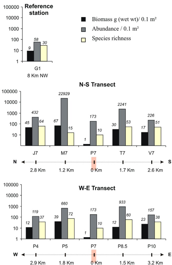
Fig. 14. Spatial variability of the major macrofaunal parameters along the E/W and N/S transects and in the control station. S, total number of species per 0.1 m 2 . (a) total abundance per 0.1 m 2 (number of individuals); (b) total biomass per 0.1 m 2 .
