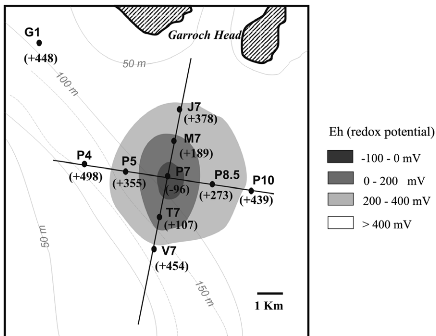
Fig. 2a. Redox potential in the surface sediment.
