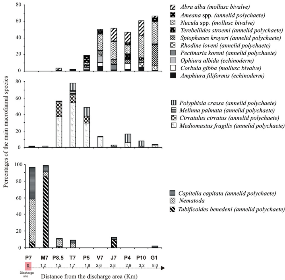
Fig. 17. Change in dominant species of benthic macrofauna (>5%) following the distance from the discharge point.
