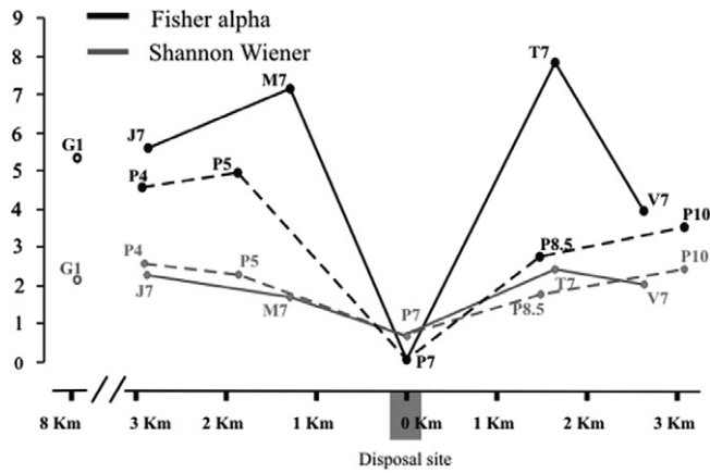
Fig. 10. Fisher alpha index and Shannon–Wiener index of benthic foraminifera along NS and WE transects.
