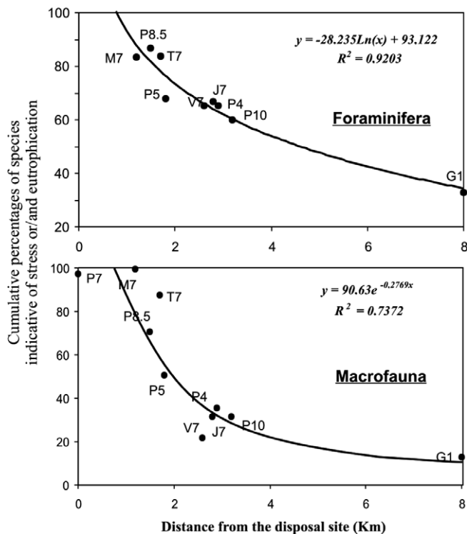
Fig. 20. Cumulative percentages of all taxa indicative of natural and/or anthropogenic eutrophication and ecosystem stress, in function of distance to the drill cutting disposal.
