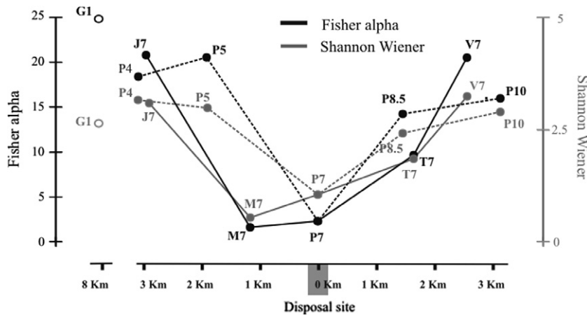
Fig. 15. Fisher alpha index and Shannon–Wiener index of macrofauna along NS and WE transects.
