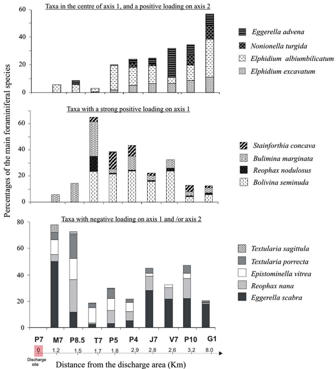
Fig. 12. Change in dominant species of total benthic foraminifera (>5%).
