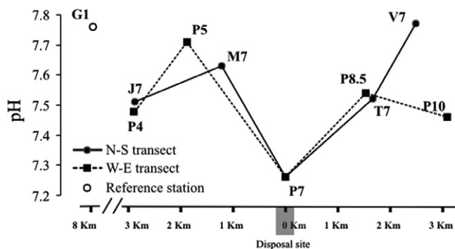
Fig. 3. Acidity of the sediment surface along the transects.
