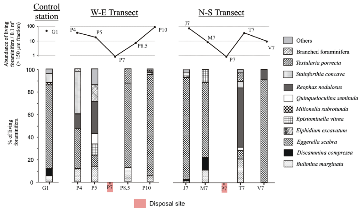
Fig. 7. Density and composition of foraminiferal faunas (>150 µm fraction) for 0.1 m 2 sediment surface.
