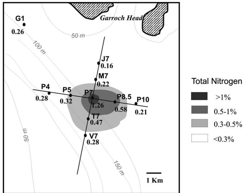
Fig. 5. Distribution of total nitrogen in the surficial sediment (%d.w.).
