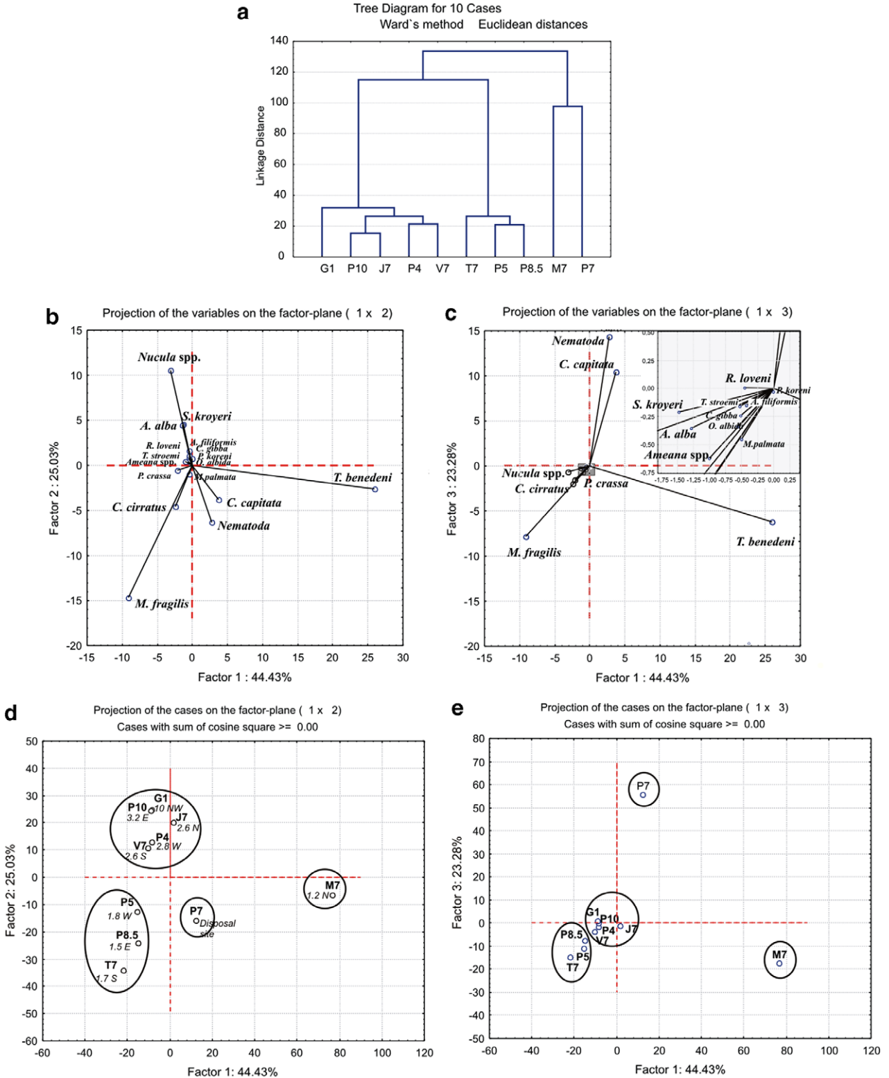
Fig. 16. PCA analysis. (a) Cluster according to Euclidean distances. (b) Projection of the variables (macrofauna) on the first two PCA axes. (c) Projection of the variables (macrofauna) on the factor-plane determined by PCA axes 1 and 3. (d) Plot of the 10 stations on the first two PCA axes, and four distinct assemblages (indicated by the dotted lines). (e) Plot of the 10 stations on the factor-plane determined by PCA axes 1 and 3.
