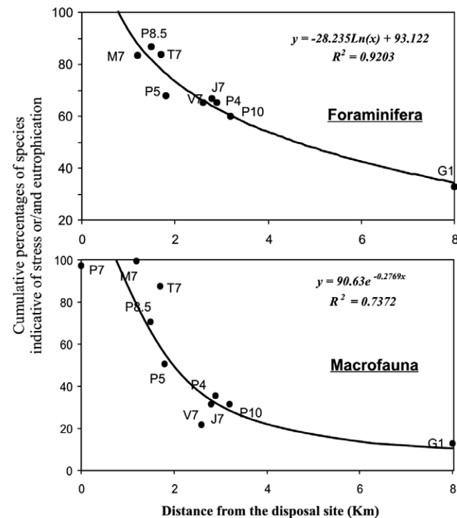
Fig. 20. Cumulative percentages of all taxa indicative of natural and/or anthropogenic eutrophication and ecosystem stress, in function of distance to the drill cutting disposal.
