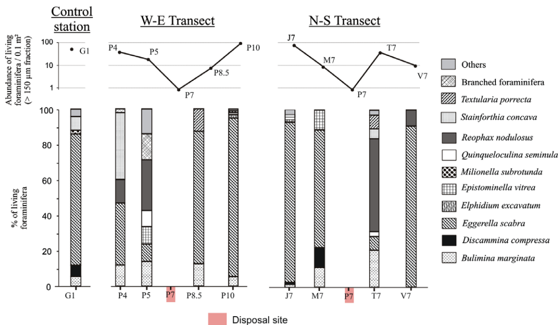
Fig. 7. Density and composition of foraminiferal faunas (>150 μm fraction) for 0.1 m 2 sediment surface.
