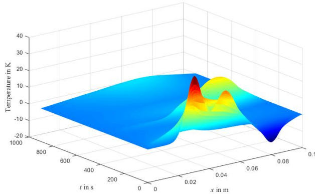
Fig. 9. Temperature evolution with control (strategy #3; \tilde{J}_{min} = 0.1 ; \tilde{J}_{max} = 0.5 ).
