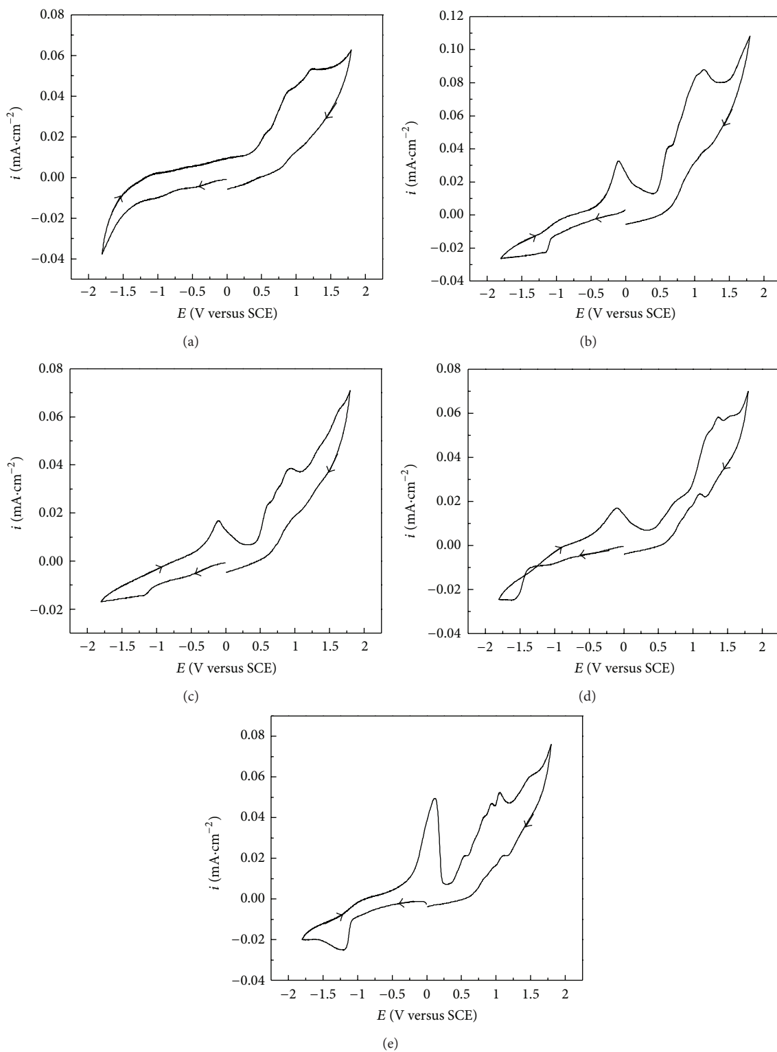
FIGURE 6: Representative cyclic voltammograms in DMF at room temperature (ionic strength: 0.1 \text{ mol L}^{-1} , \text{Bu}_4\text{NClO}_4 , i in mA, \nu = 100 \text{ mVs}^{-1} ) of H_2L (a), [Co(H_2L)]^{4+} (b), [(CoCl_2)_2(H_2L)]^{4+} (c), [Ni(H_2L)]^{4+} (d), and [(NiCl_2)_2L]^{2+} (e) in the -1.80 to +1.80 range.
