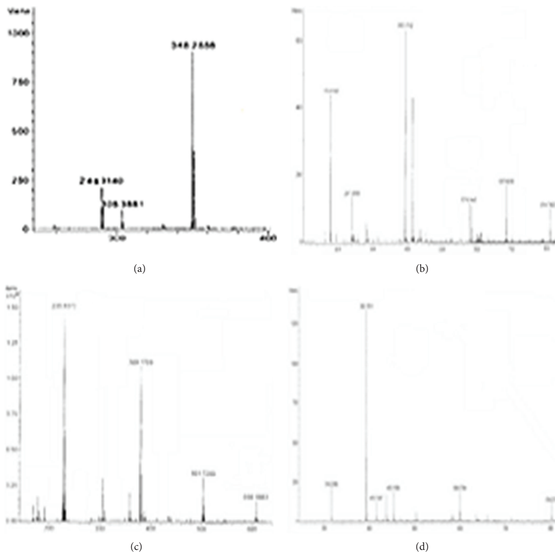
FIGURE 2: Mass spectra of H 2 L (a), ([Co(H 2 L)] 4+ ) 2 (b), [(CoCl 2 ) 2 (H 2 L)] 4+ (c), and ([Ni(H 2 L)] 4+ ) 2 (d).
