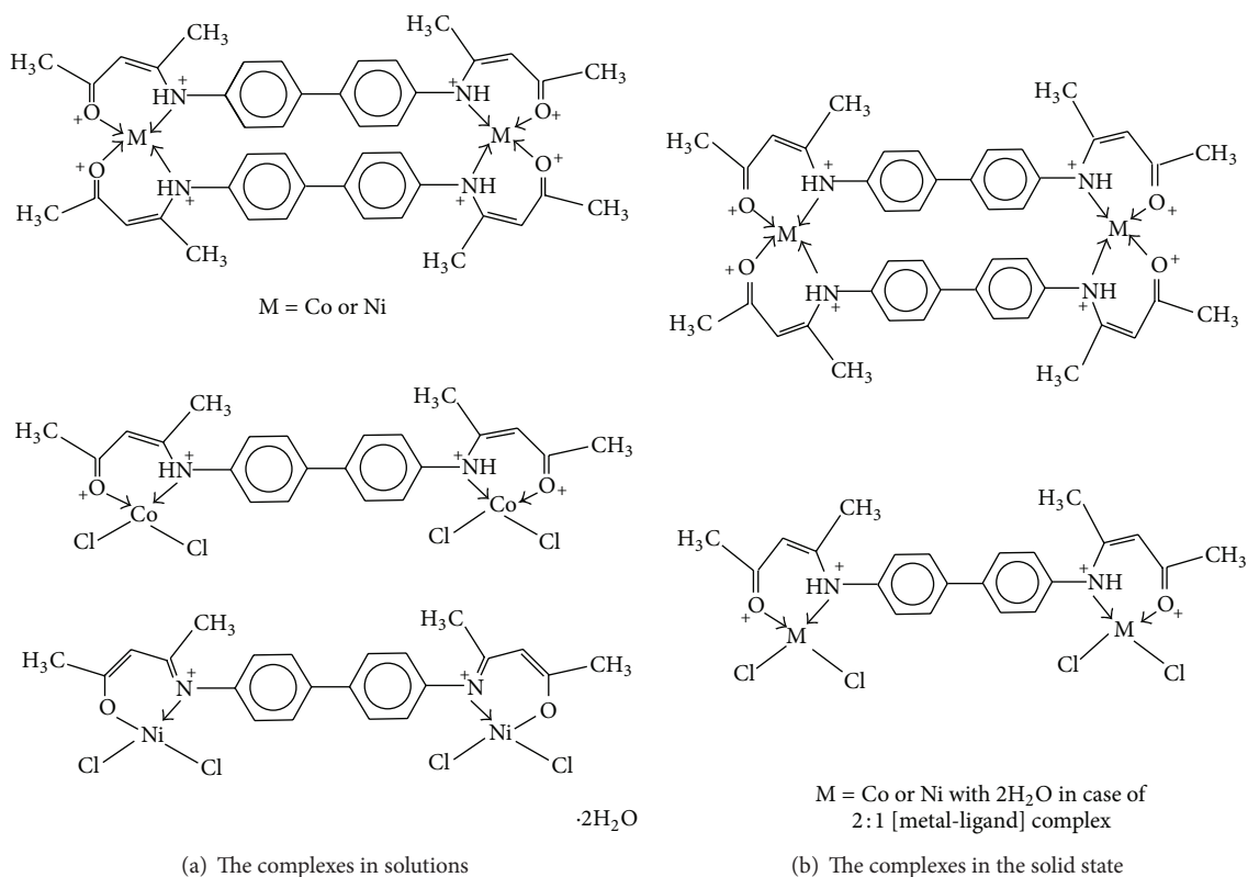
FIGURE 5: Proposed structures for Co II and Ni II complexes either in solution (a) or in solid state (b).
