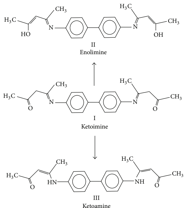
FIGURE 3: Ketoimine form of the Schiff base ligand H_2L in solid state and its ketoamine or enolimine tautomer form when dissolved in organic solvent.
