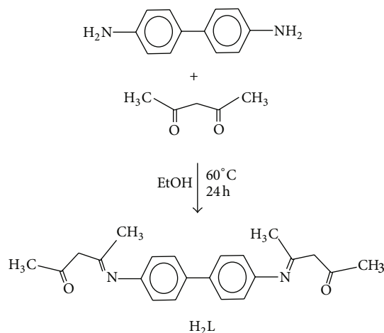
FIGURE 1: Synthetic route of the Schiff base ligand \text{H}_2\text{L} .
