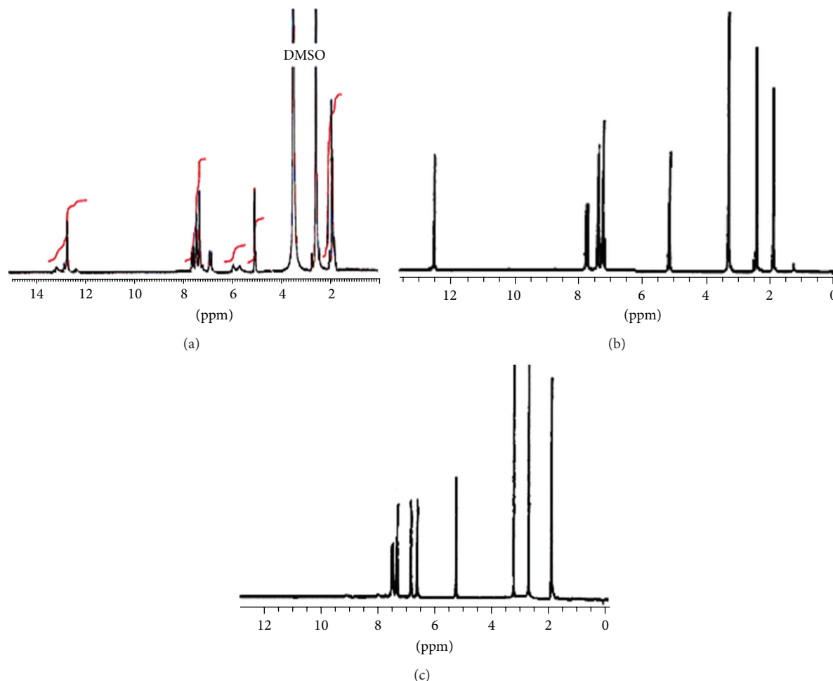
FIGURE 4: ^1\text{H} NMR spectra of \text{H}_2\text{L} (a), [(\text{Ni}(\text{H}_2\text{L}))^{4+}]_2 (b), and [(\text{NiCl}_2)_2\text{L}]^{2+} (c) in \text{DMSO-D}_6 solution and in the \delta 0–13 ppm range.
