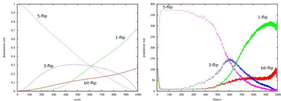
Fig. 1. Domination rates evolution for the 1000-bits One-Max problem.
