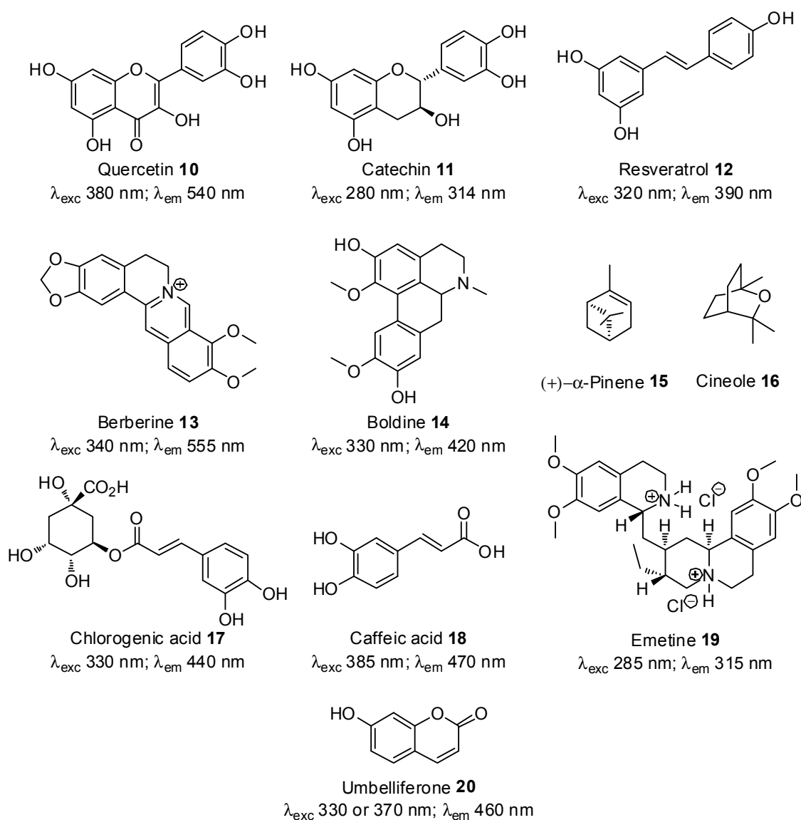
Figure 3. Tested NPs 10–20 and their fluorescent excitation and emission wavelengths in water.
