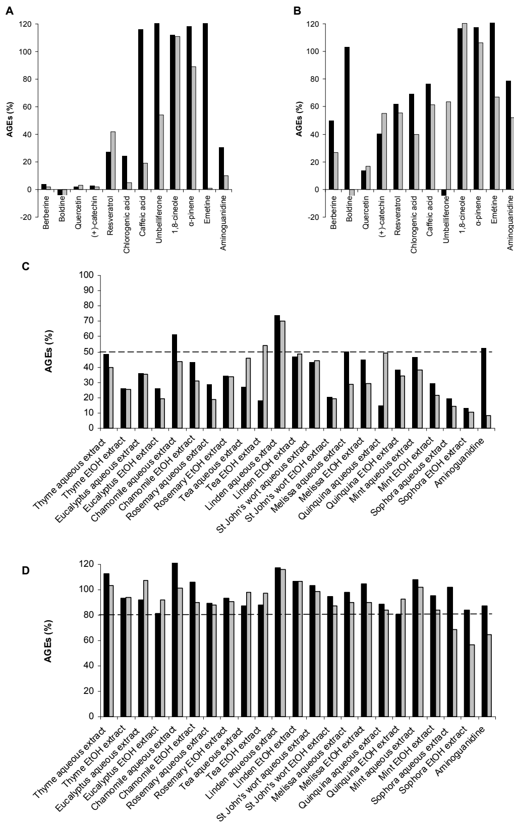
Figure 4. Vesperlysin-like (black) and pentosidine-like (grey) AGE formation in the presence of NPs ( A : 1 mg/mL; B : 0.1 mg/mL) or plant extracts ( C : 1 mg/mL; D : 0.1 mg/mL).
