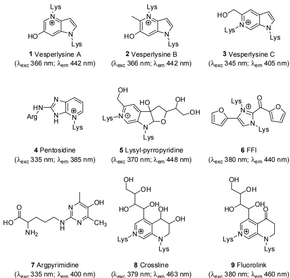
Figure 1. Structures of the main fluorescent AGEs 1–9 and their fluorescent properties in neutral aqueous media [31–36].
