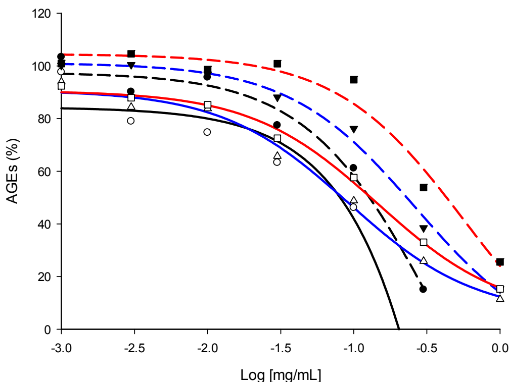
Figure 6. Dose-effect curves for vesperlysines-like AGE (dotted) and pentosidine-like AGE (bold) formation in the presence of quinquina EtOH extract (Black), sophora EtOH extract (Blue) or sophora aqueous extract (Red).
