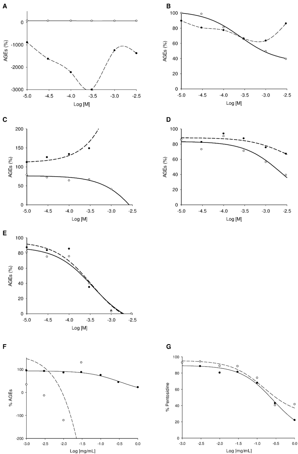
Figure 5. Dose-effect curves for vesperlysines-like AGE (dotted) and pentosidine-like AGE (bold) formation in the presence of umbelliferone 20 (A), caffeic acid 18 (B), emetine 19 (C) or aminoguanidine (D) or quercetin 10 (E) as well as dose-effect curves for vesperlysines-like AGE (F) and pentosidine-like AGE (G) formation in the presence of Mammea neurophylla fruit methanolic extract with (dotted) or without (bold) umbelliferone 20 (10% m/m).
